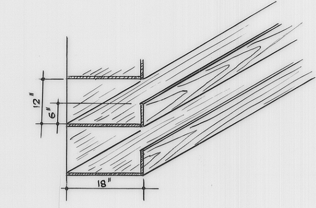
DETAILS OVERSIZE PLAN SHELVES
