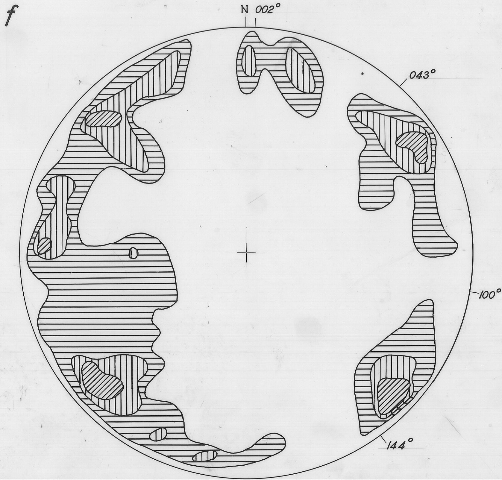
EQUAL AREA PROJECTIONS OF STRUCTURAL ELEMENTS (I)
