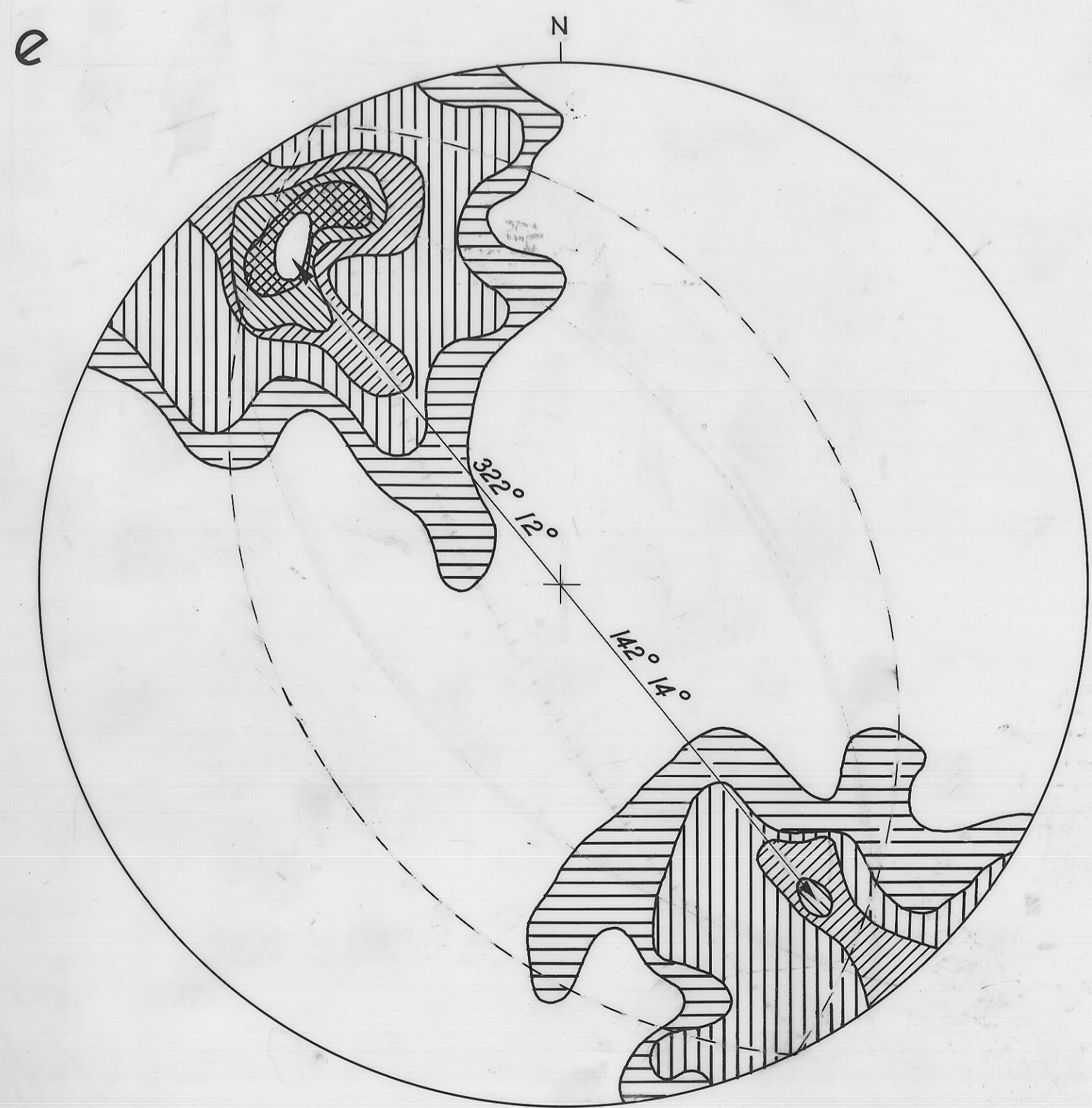
EQUAL AREA PROJECTIONS OF STRUCTURAL ELEMENTS (I)
