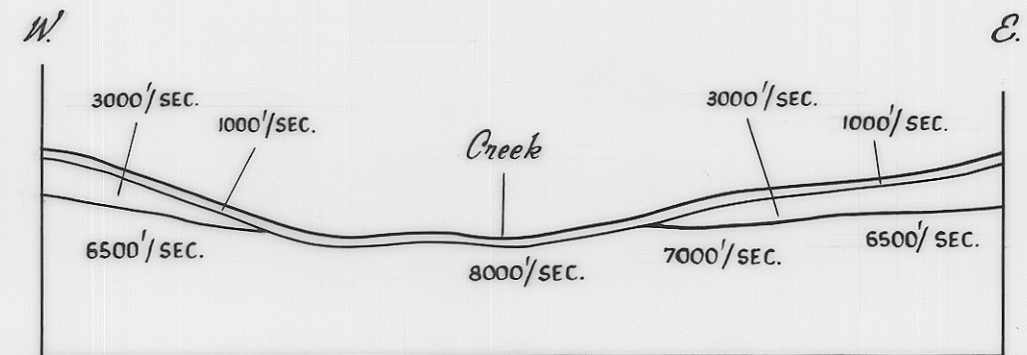
SKETCH SECTION ALONG CENTRELINE OF SEISMIC TRAVERSE NOT TO SCALE
