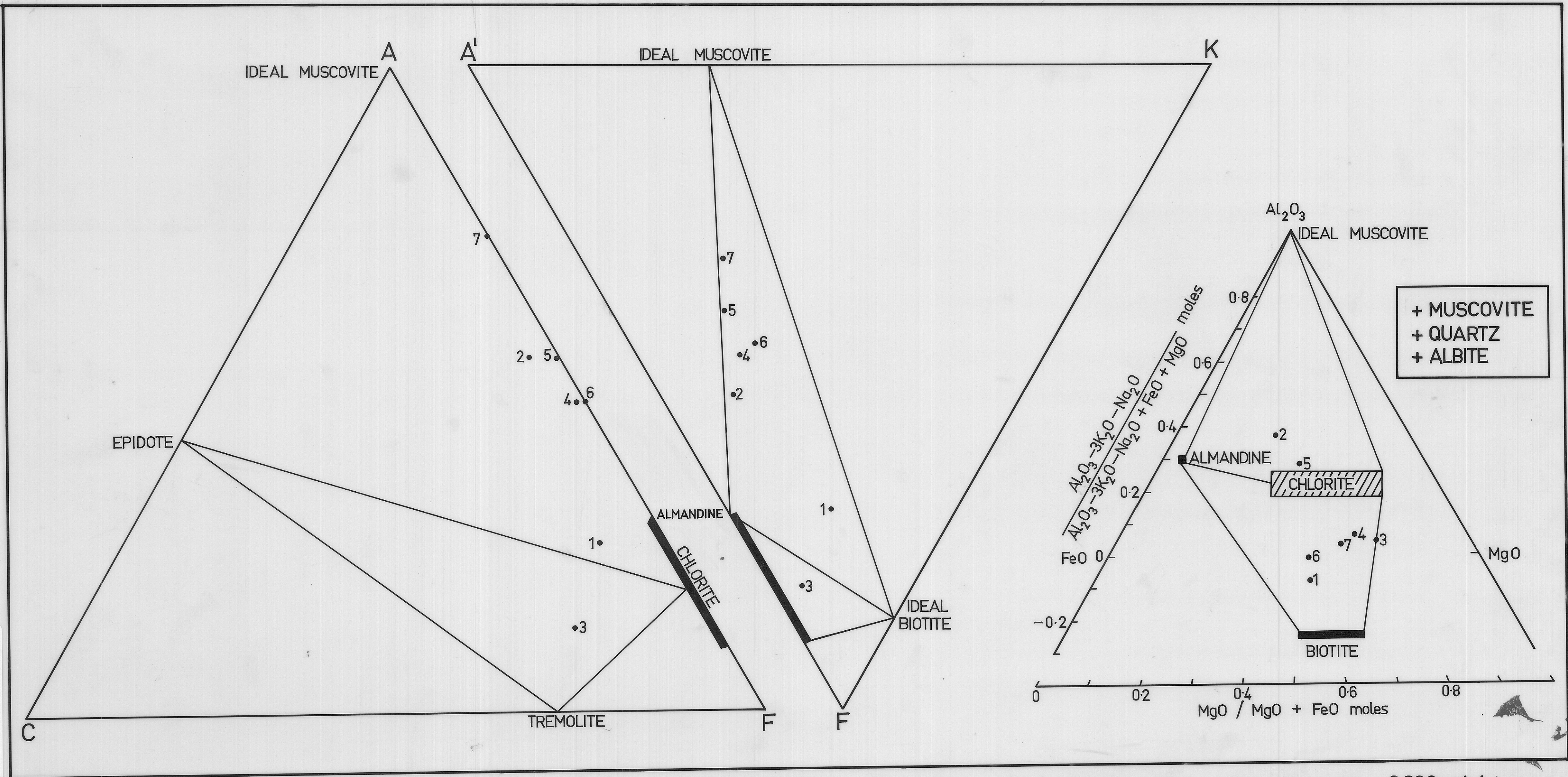
Metamorphic Facies Diagram PE Bradburn (Mackintosh). ACF, A'KF and AFK plots
