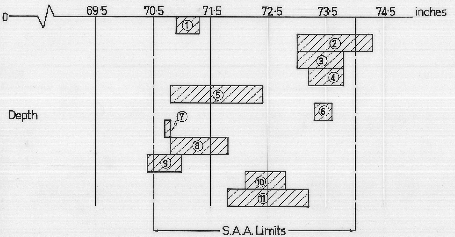
COMPARISON OF BRICK DIMENSIONS WITH SPECIFICATION REQUIREMENTS R605 (DEC 1969)
