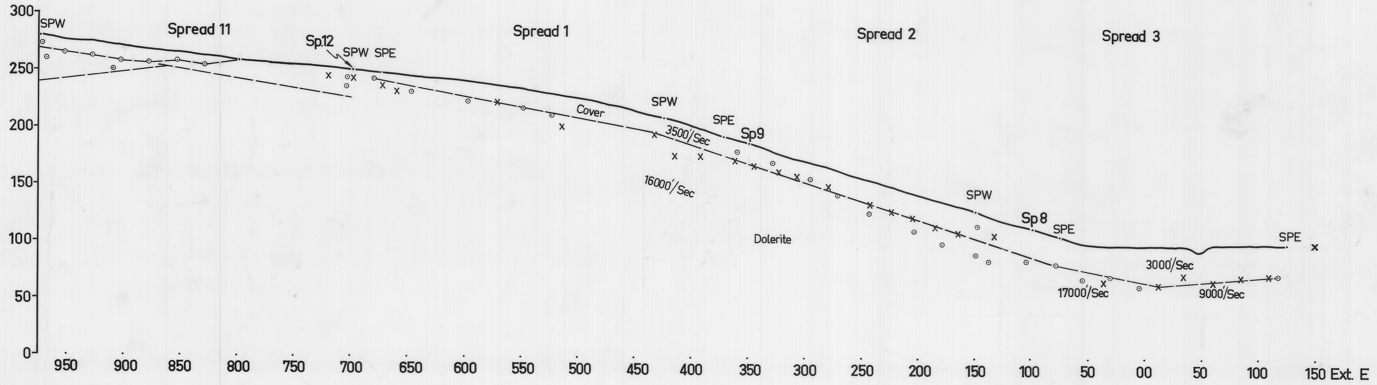
SEISMIC LINE D QUARRY SITE — KINGSTON
