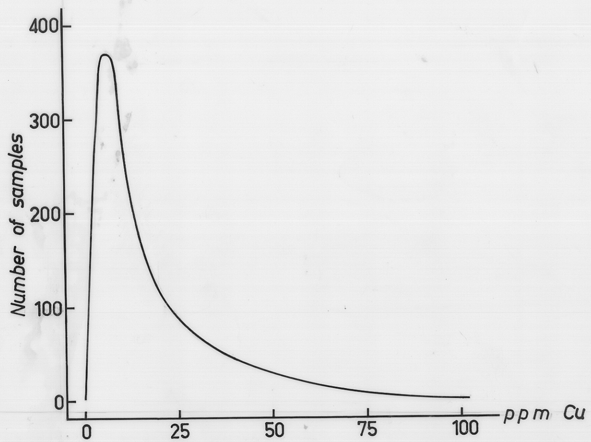
FREQUENCY AND CUMULATIVE FREQUENCY CURVES FOR LEAD ZINC AND COPPER IN SOILS FROM OLIVER HILL
