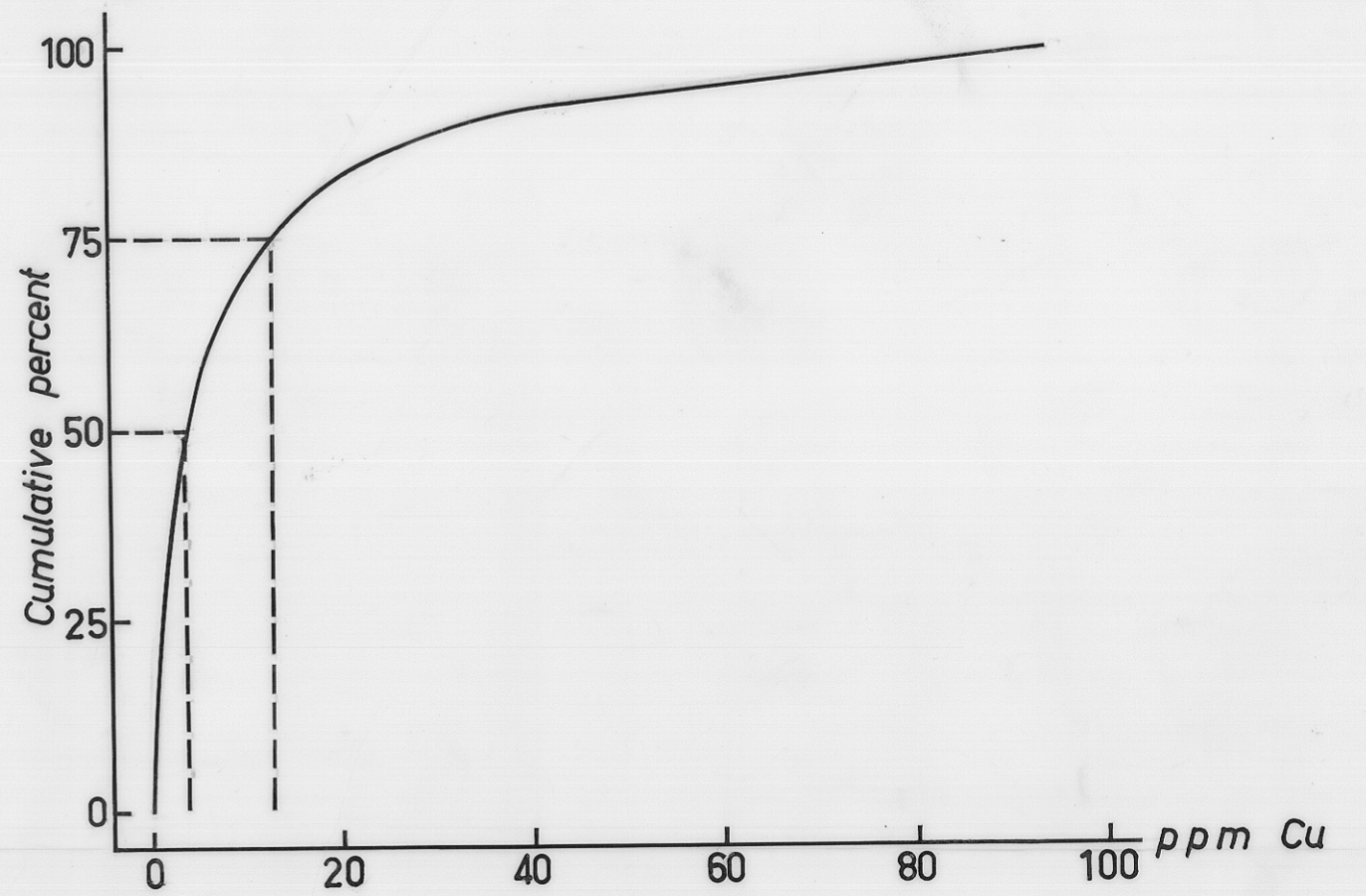
FREQUENCY AND CUMULATIVE FREQUENCY CURVES FOR LEAD ZINC AND COPPER IN SOILS FROM OLIVER HILL
