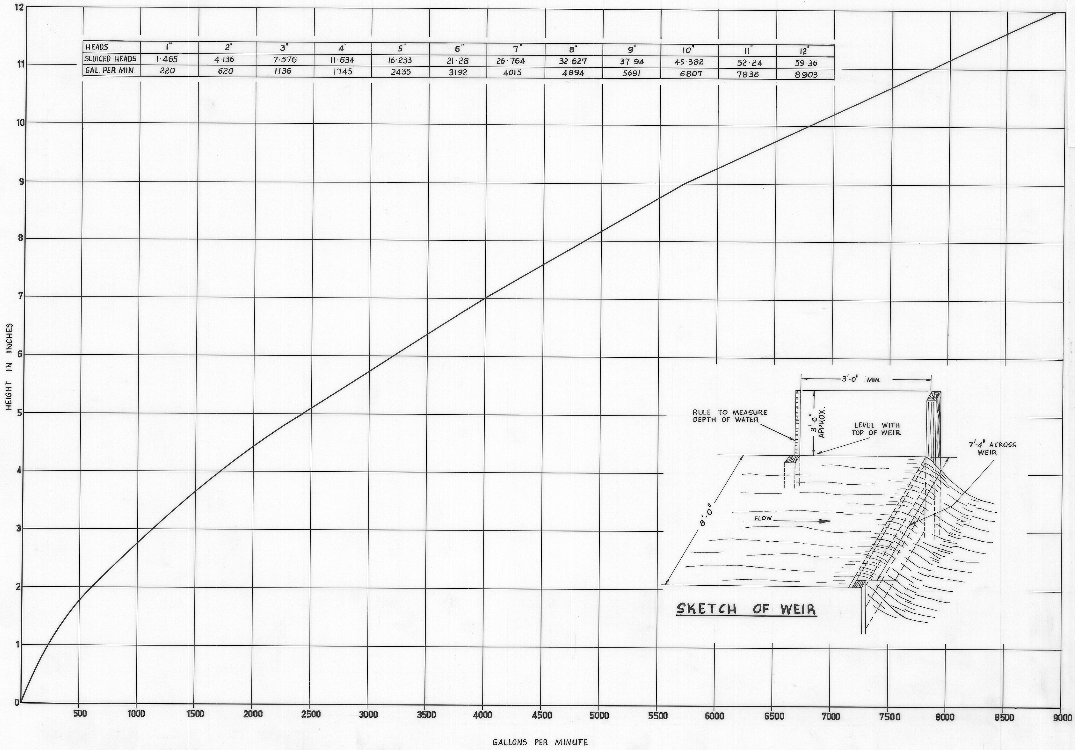
MEASURING FLOW IN SLUICE BOX—PIONEER MINE
