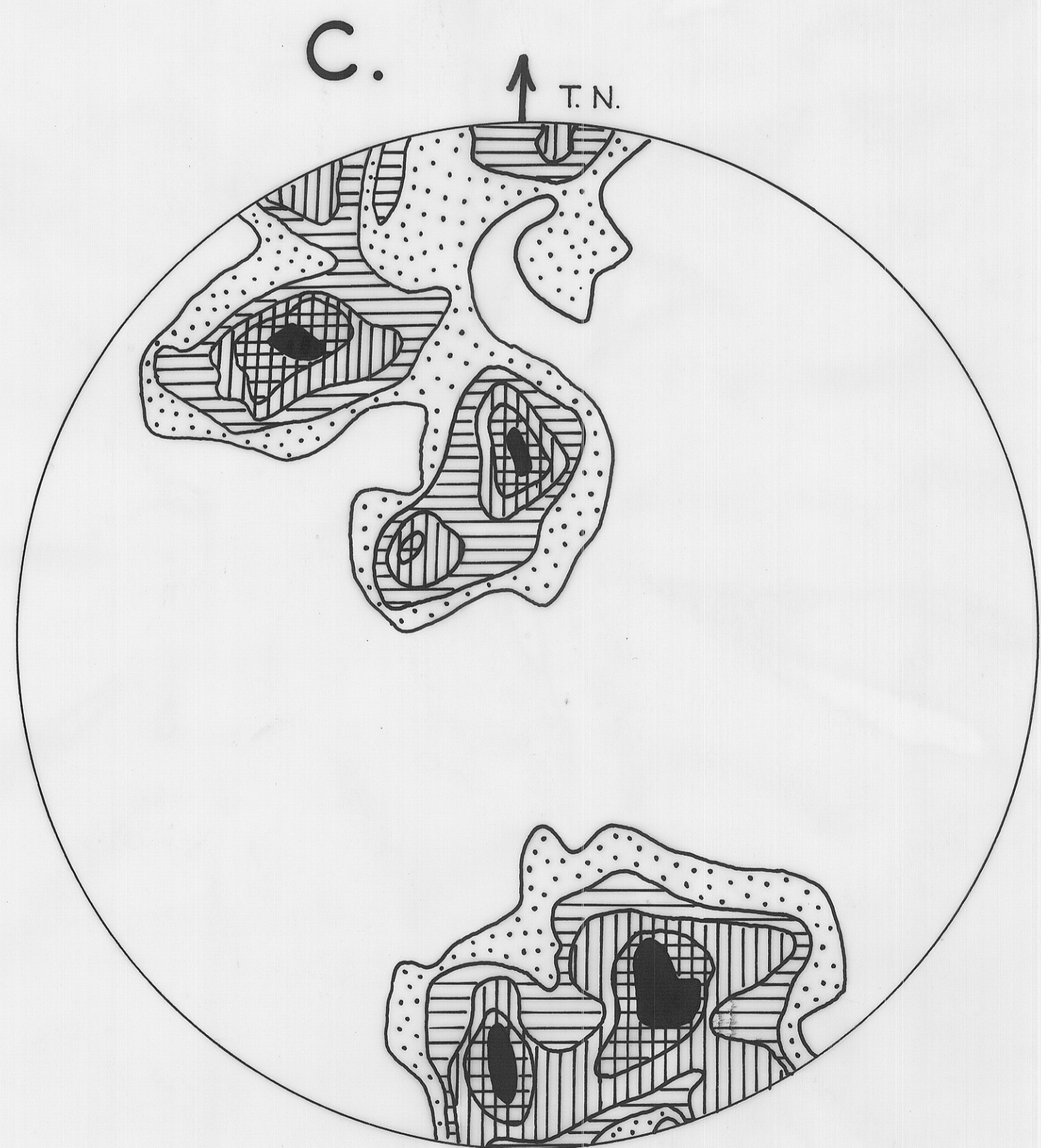
C. BEDDING ORIENTATION MT. BISCHOFF SEQUENCE 200 \pi ; 2-3-4-5-6 %
