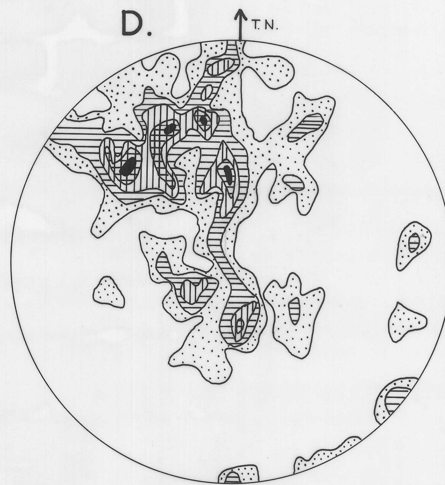
D. BEDDING ORIENTATION WARATAH RIVER SEQUENCE 150 \pi ; 2-3-4-5-6 %
