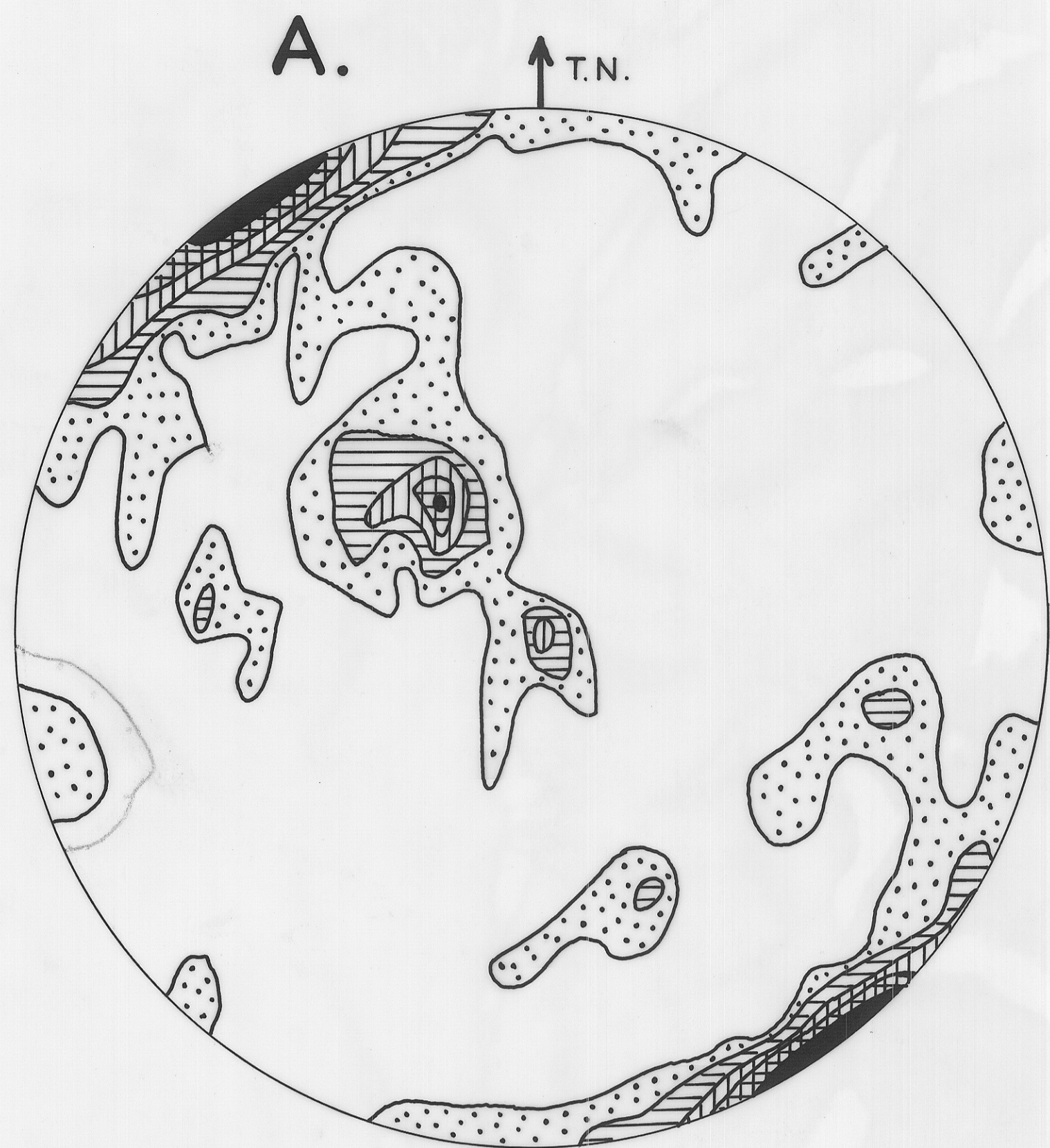
A. AXIAL SURFACES OF FOLDS MT. BISCHOFF SEQUENCE 100 \pi ; 2-3-4-5-6 %
