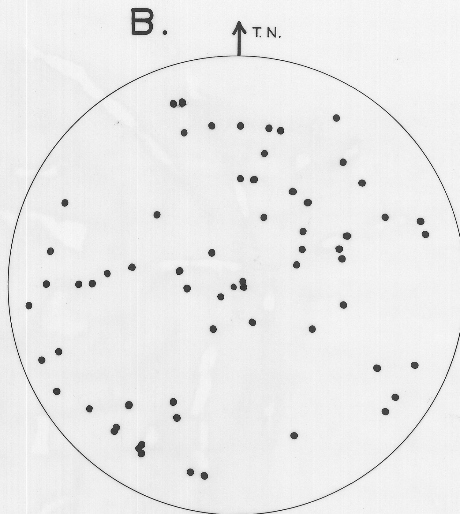
B. AXES OF FOLDS MT. BISCHOFF SEQUENCE 65 \pi
