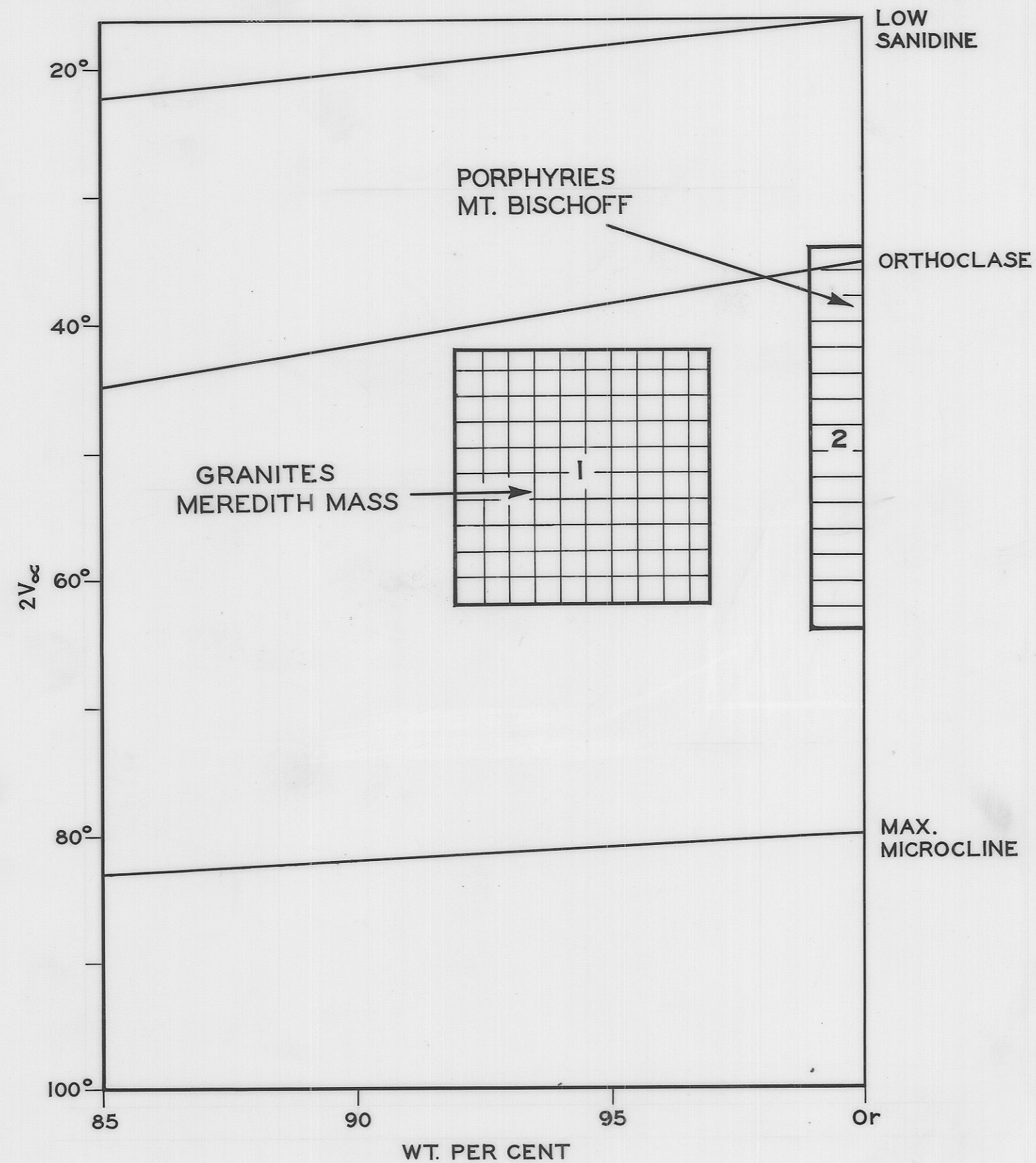
RANGE IN OPTIC AXIAL ANGLES AND COMPOSITION OF ALKALI FELDSPARS PLOTTED ON DIAGRAM OF TUTTLE (1952) AS MODIFIED BY EMELEUS & SMITH (1959)
