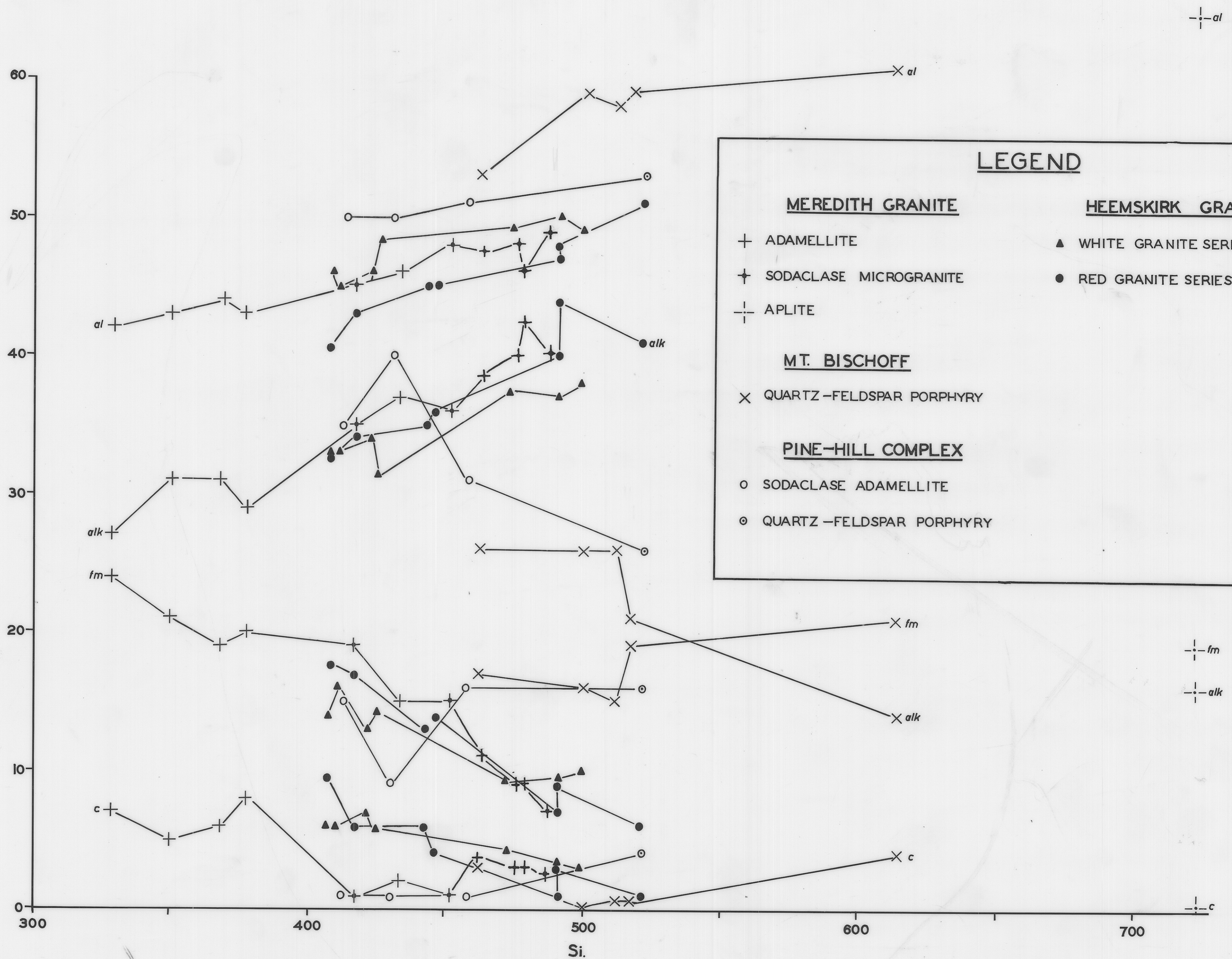
VARIATION DIAGRAM (NIGGLI VALUES) OF GRANITIC ROCKS WEST COAST TASMANIA
