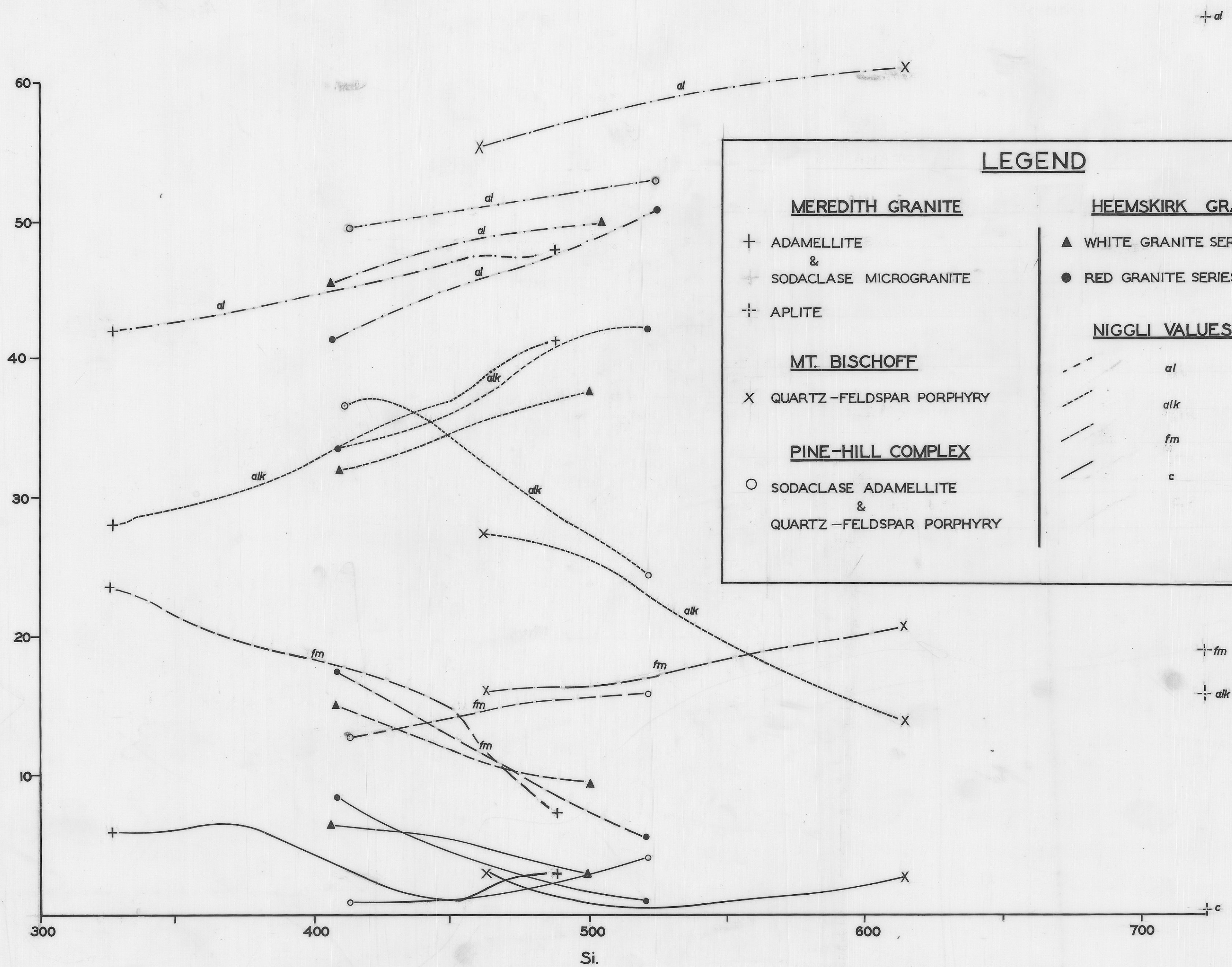
GENERALISED CHEMICAL TRENDS OF GRANITIC ROCKS WEST COAST TASMANIA
