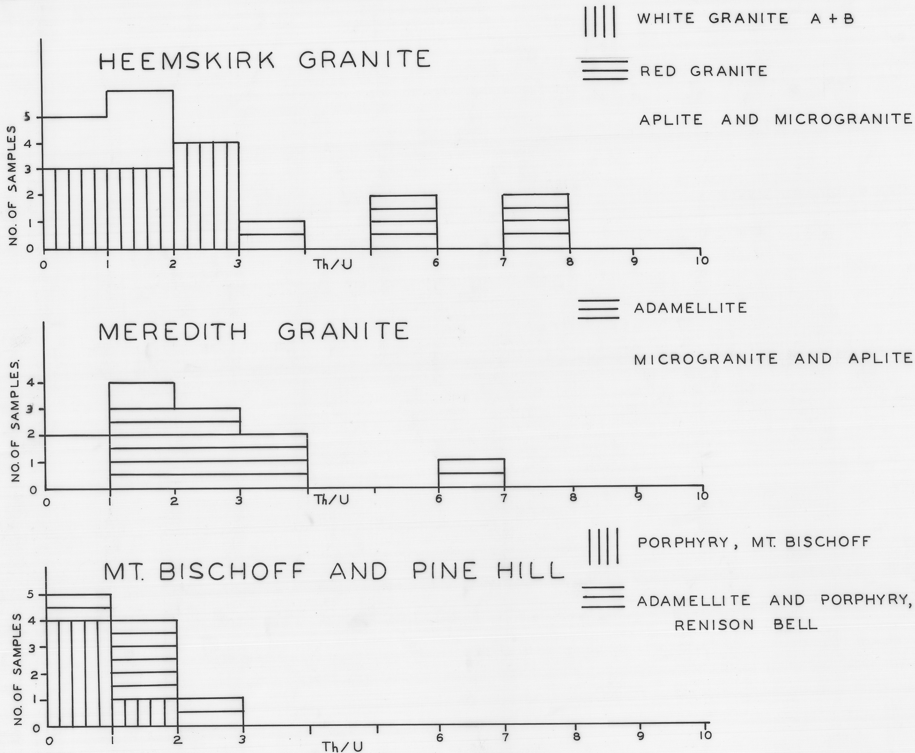
A. HISTOGRAMS SHOWING FREQUENCY OF Th/U RATIOS.
