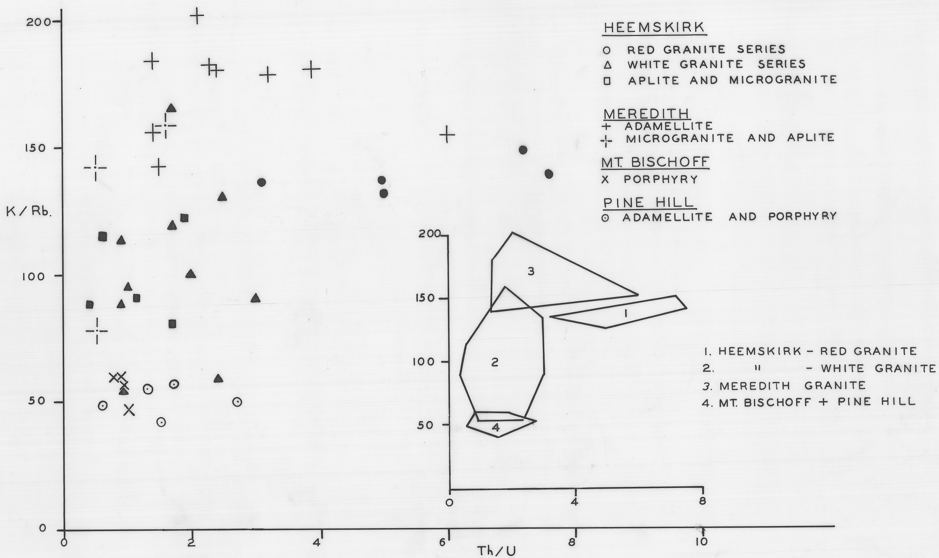
B. PLOT OF Th/U VS. K/Rb IN GRANITIC ROCKS.
