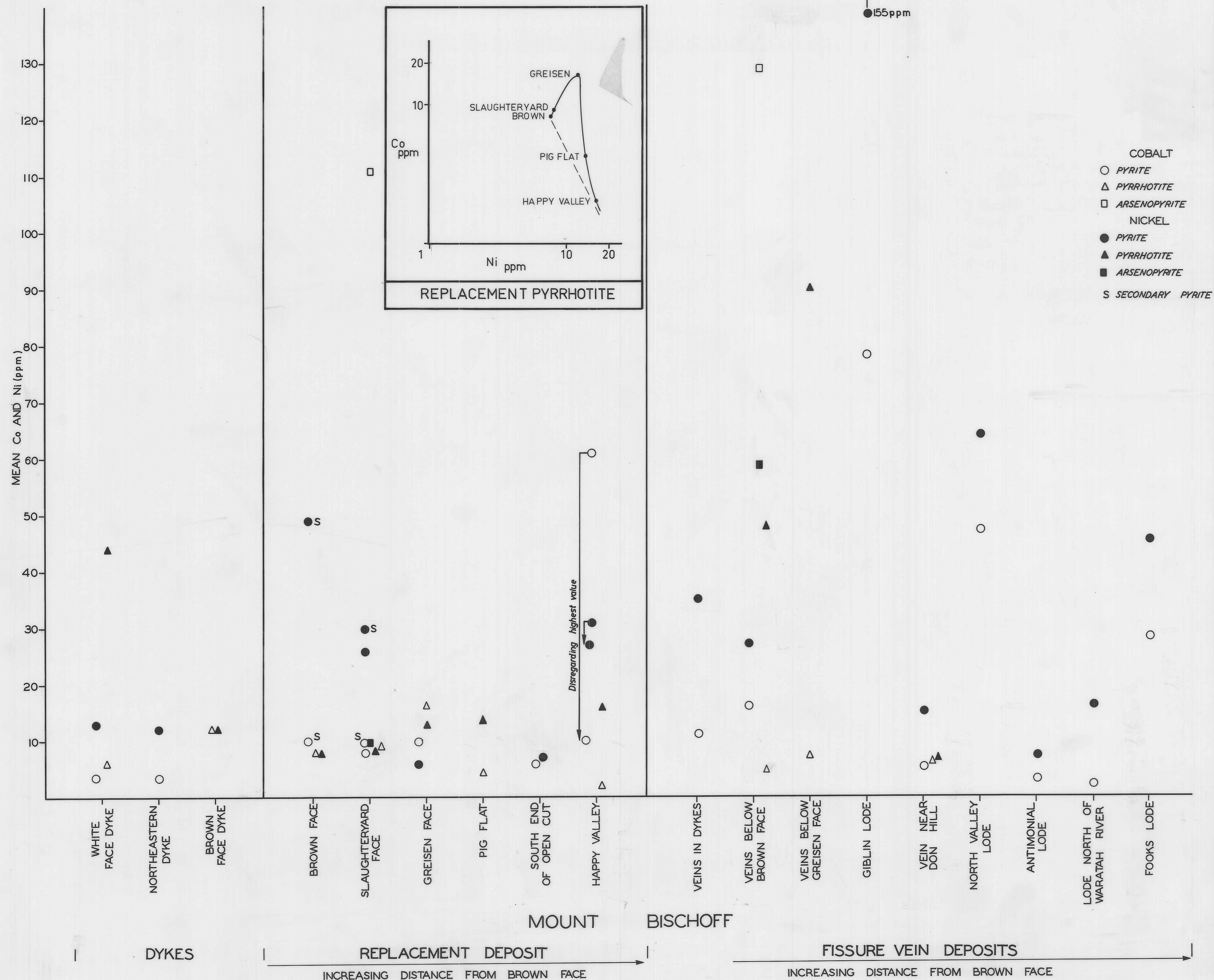
DISTRIBUTION OF Co AND Ni IN Fe-SULPHIDES MT. BISCHOFF AND RENISON BELL
