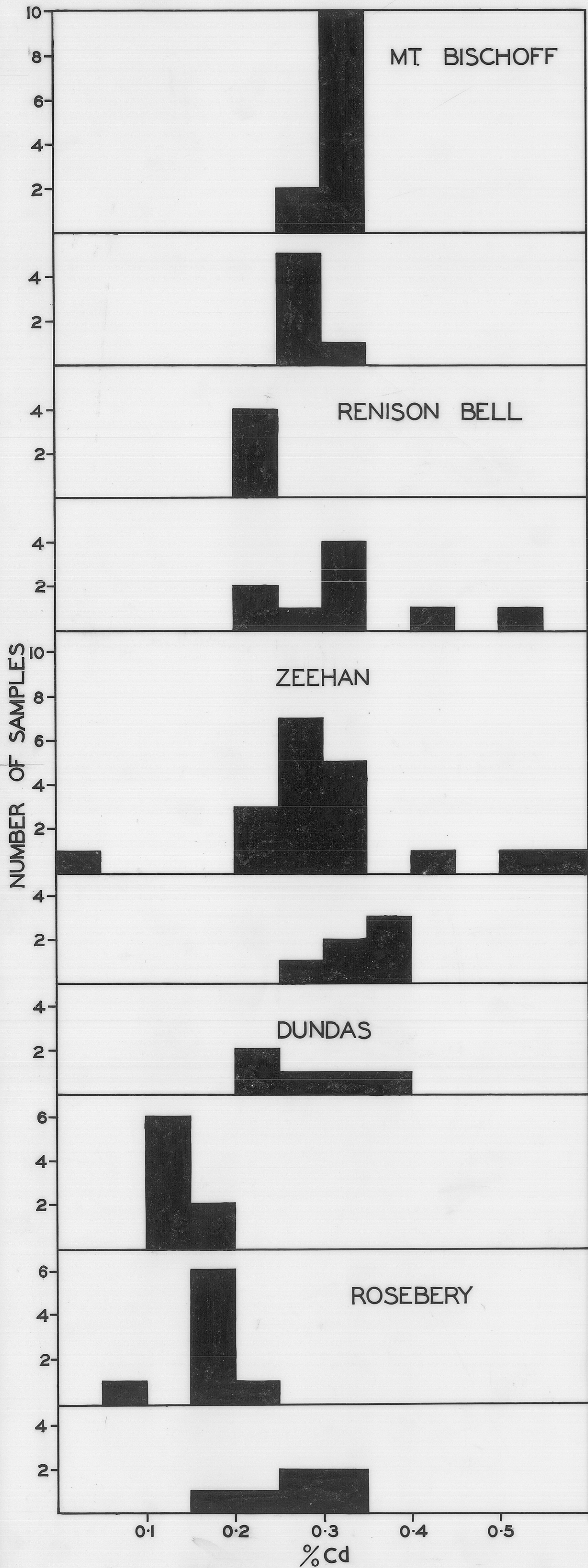
%CADMIUM IN SPHALERITE
