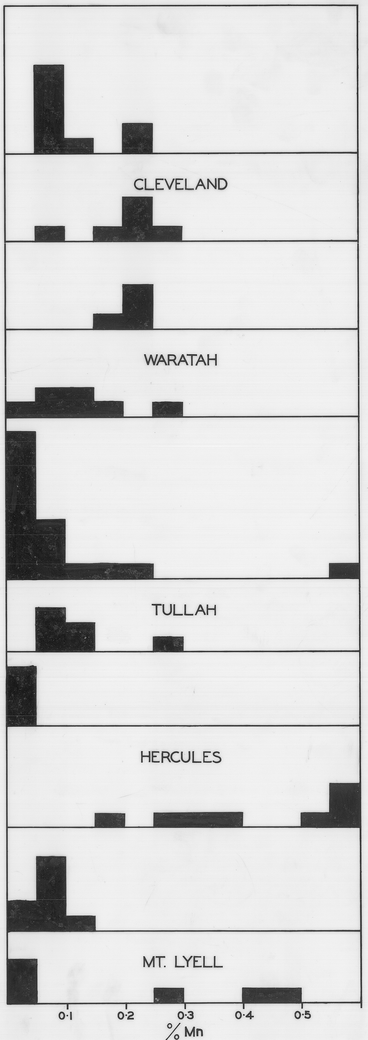
%MANGANESE IN SPHALERITE
