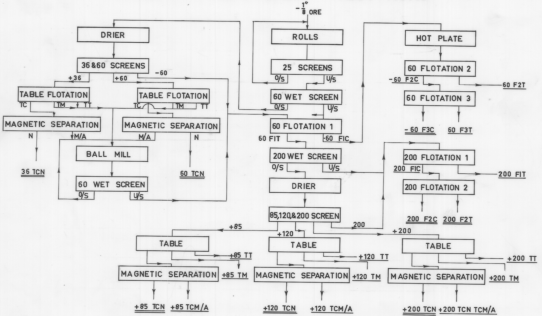
FIGURE 1 FLOW SHEET TEST NO.10
