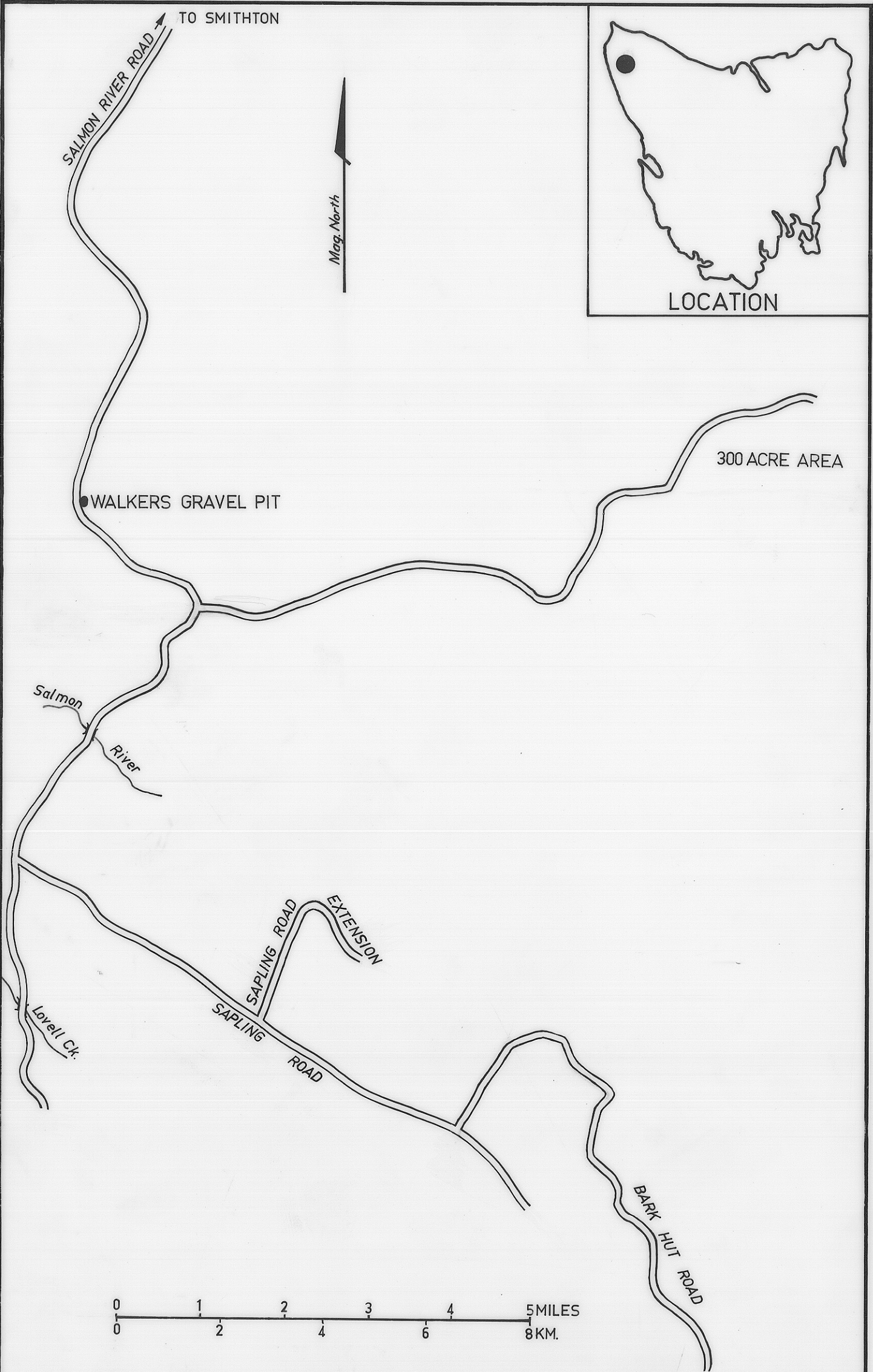
LOCALITY MAP: CHROMITE-BEARING GRAVEL DEPOSITS N. W. TASMANIA
