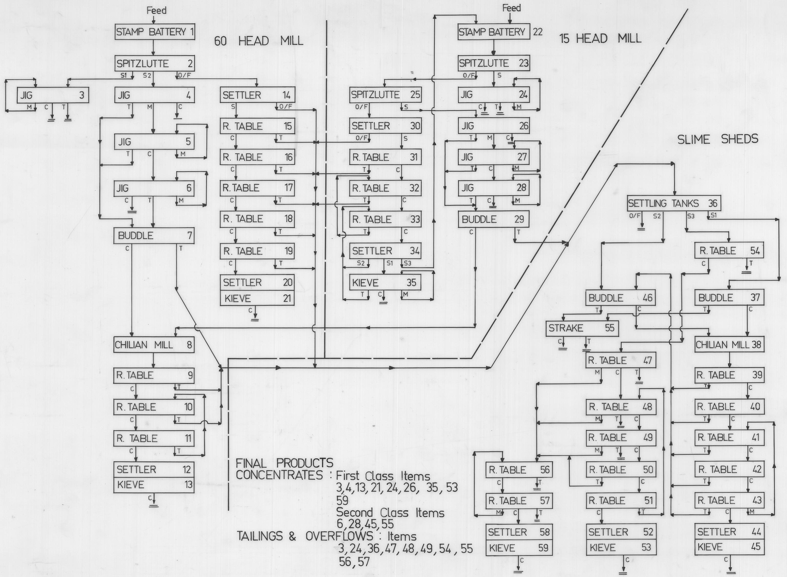
Mt. BISCHOFF TIN MINING Co. Reg. TIN CONCENTRATOR FLOWSHEET, WARATAH 1904 (Source : Herman , H.) COMPRISING : 60 Head Mill ( Items 1-21 ) 15 Head Mill ( Items 22-35 ) Slime Sheds ( Items 36-59 )
