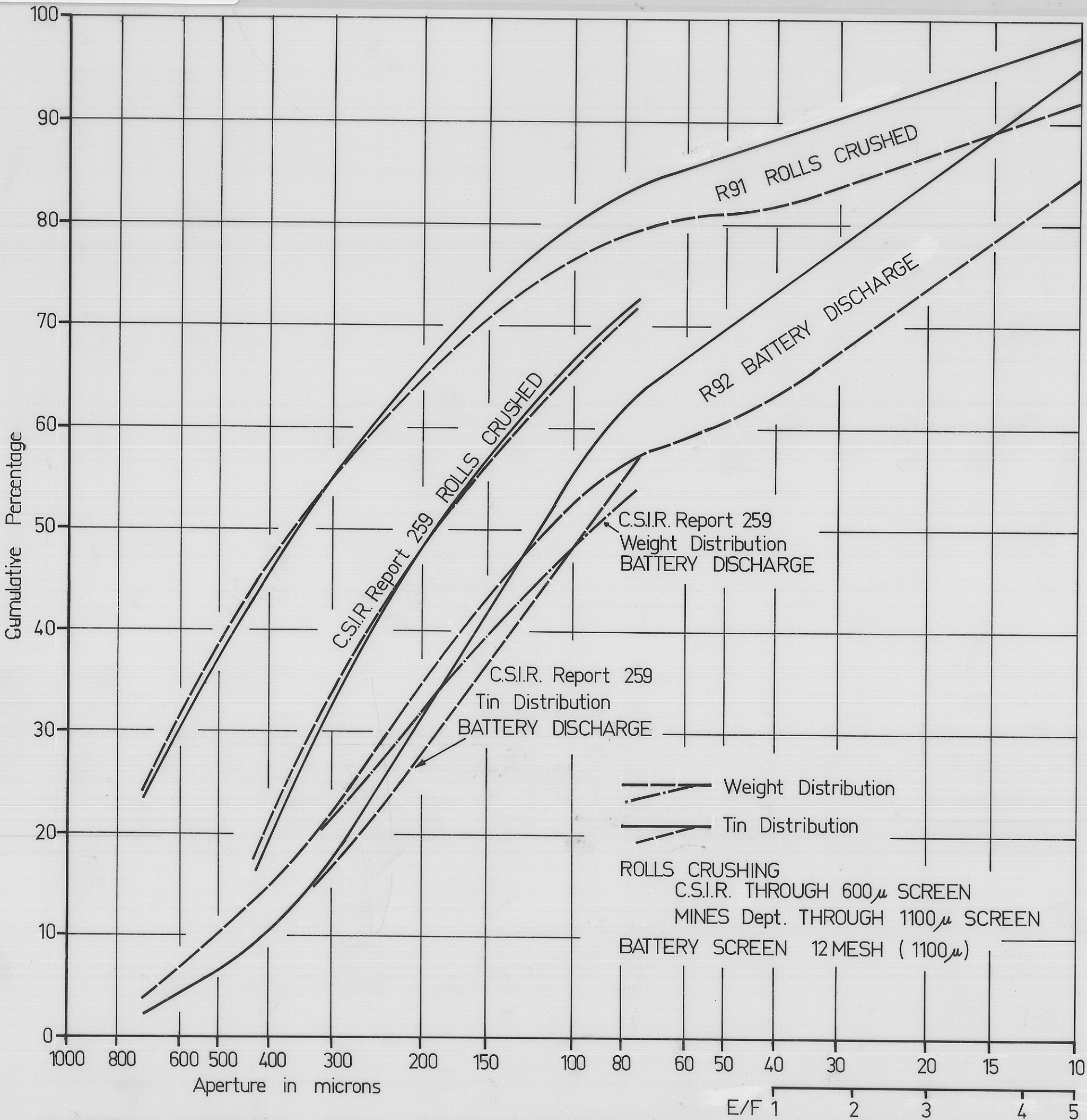
NORTH VALLEY MILL - 1943 - WEIGHT AND TIN DISTRIBUTION BATTERY DISCHARGE ( R92 & C.S.I.R. Rep. 259 ) ROLLS CRUSHING AT MINES Dept. LABORATORY (R91) ROLLS CRUSHING AT C.S.I.R. LABORATORY, MELBOURNE (Rep.259)
