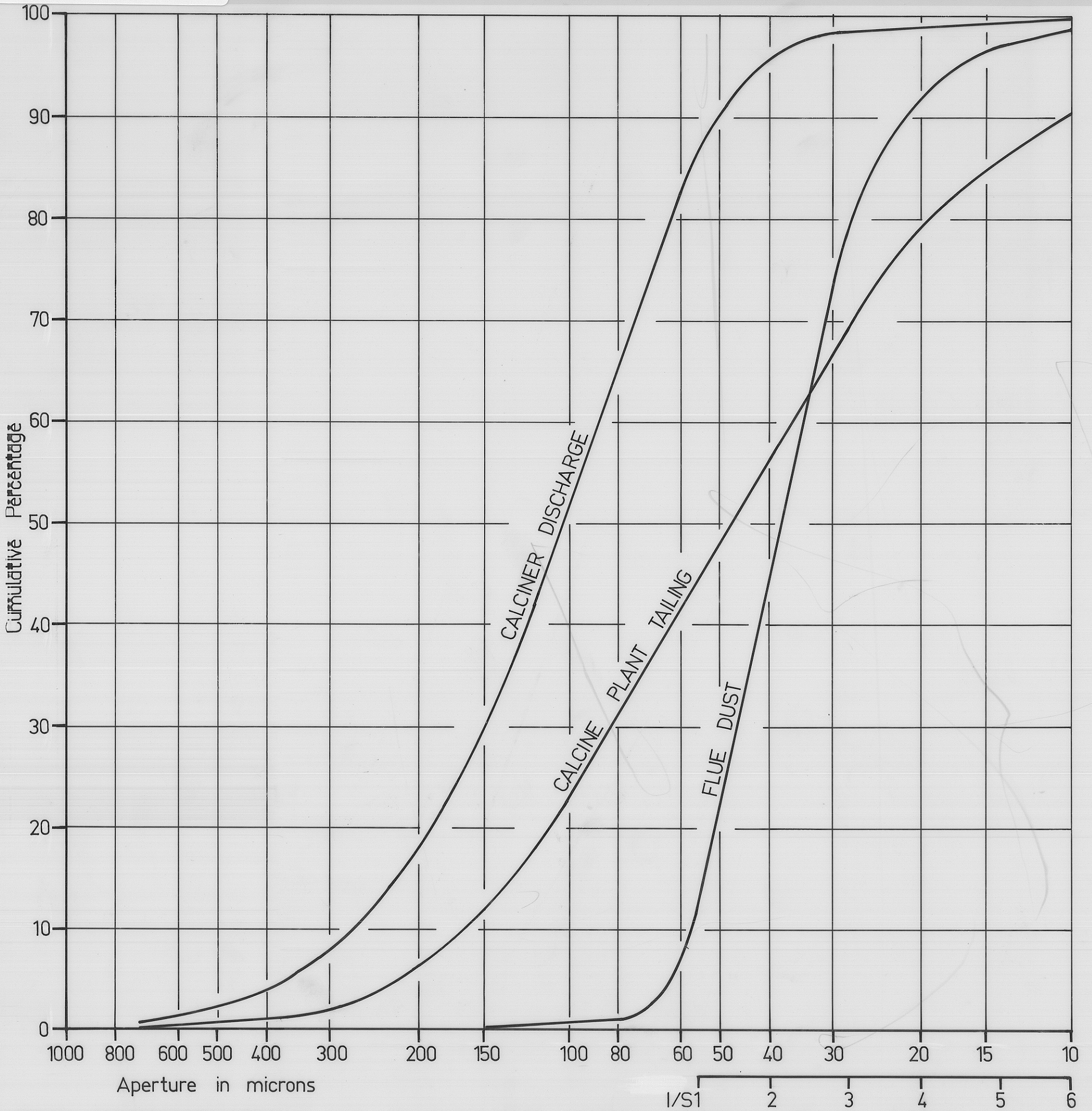
TIN DISTRIBUTION IN CALCINER PRODUCTS - 1944 - R108
