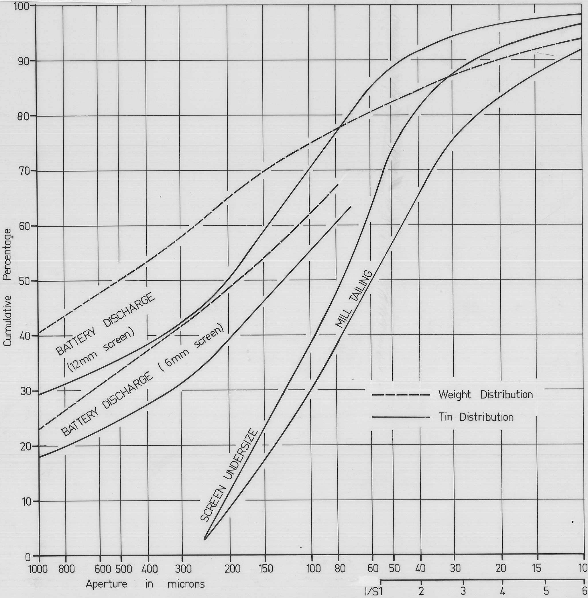
WARATAH MILL - GREISEN ORE - SAMPLING TESTS - MAY 1947 - R195 BATTERY DISCHARGE - Weight & Tin Distributions - 6 & 12 mm Battery Screens HUMMER SCREEN UNDERSIZE - Tin Distribution MILL TAILING - Tin Distribution
