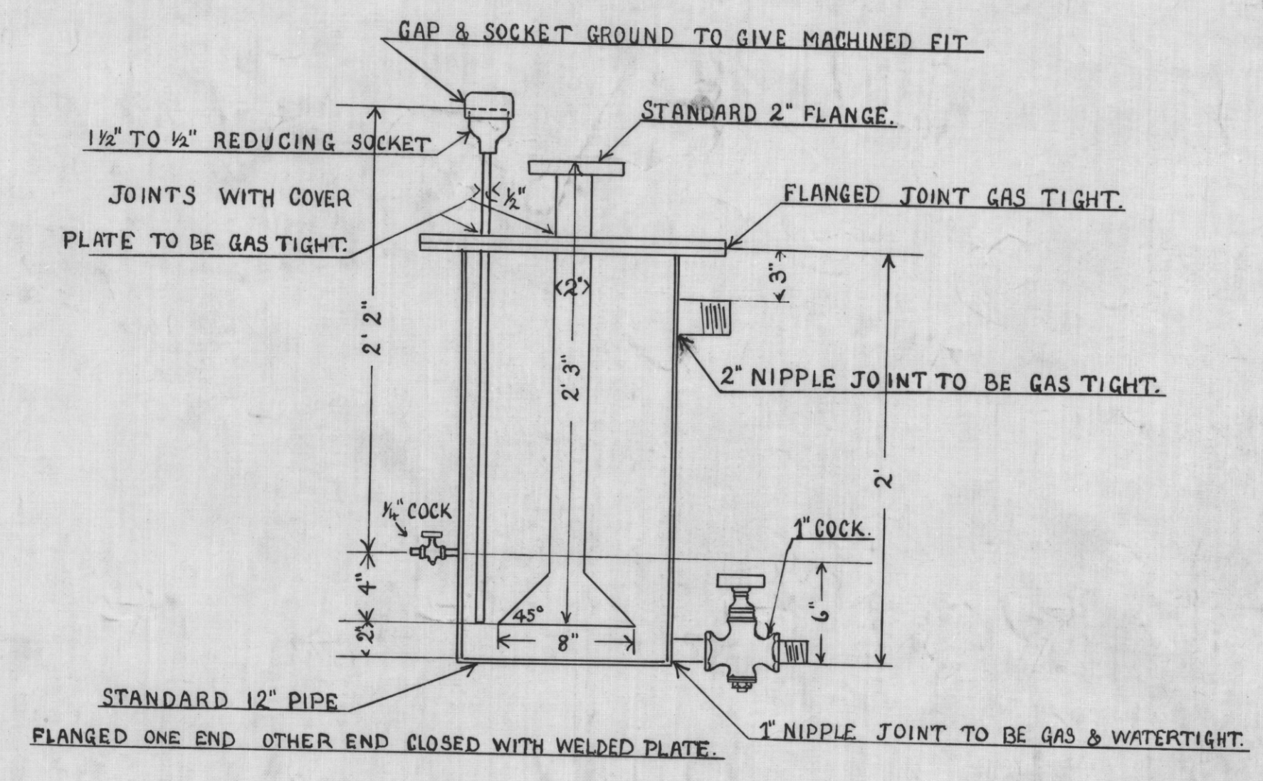
SAFETY TRAP FOR GAS LINE. MAKE 1.
