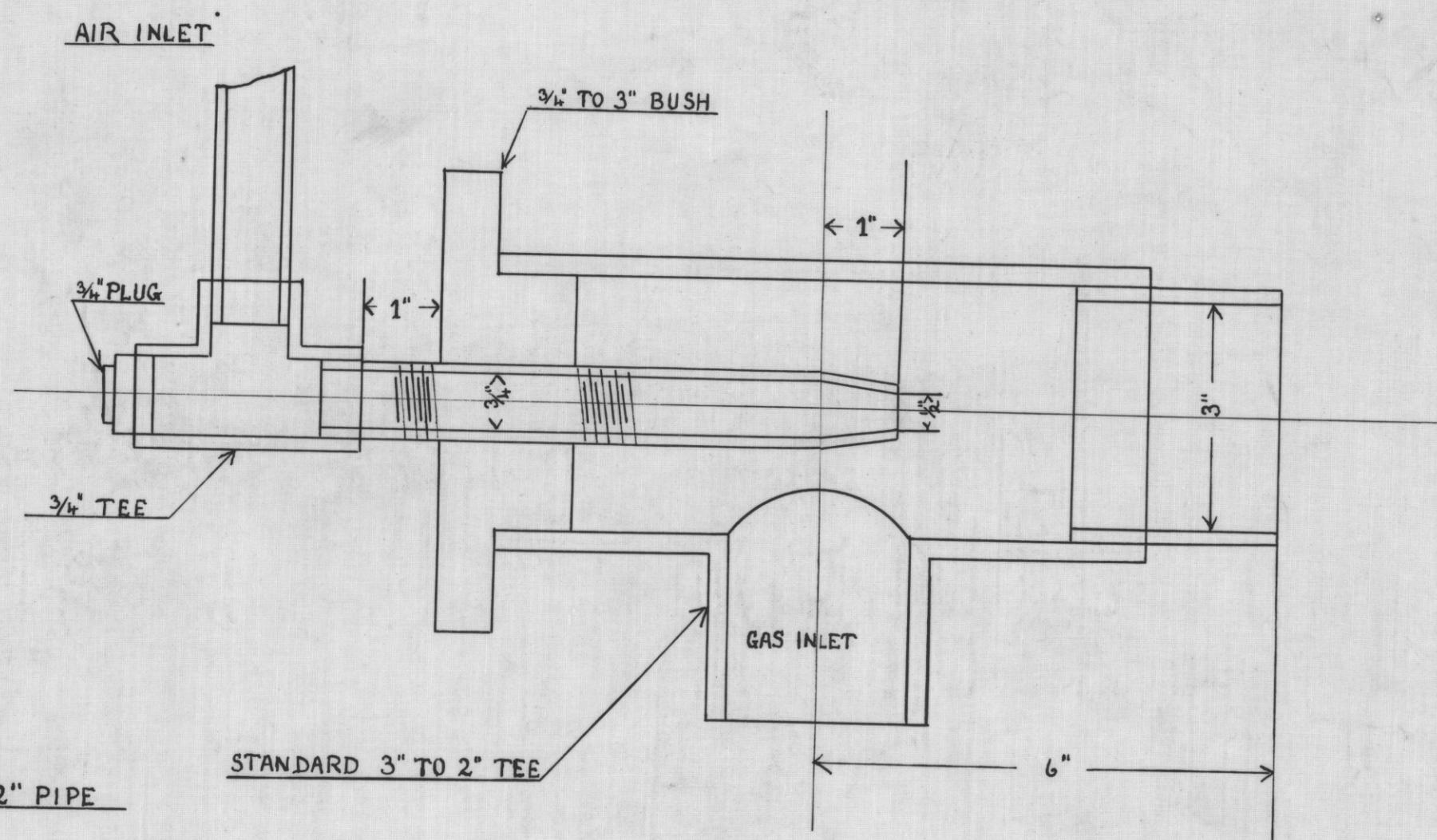
GAS BURNER FOR GAS AT ATMOSPHERIC PRESSURE. MAKE 1.
