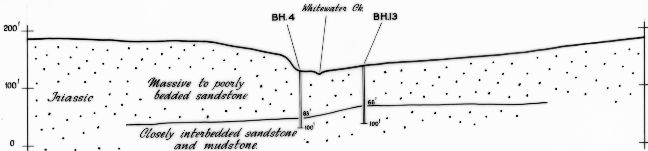
CROSS SECTION C-D LOWER DAMSITE - WHITEWATER CK.
