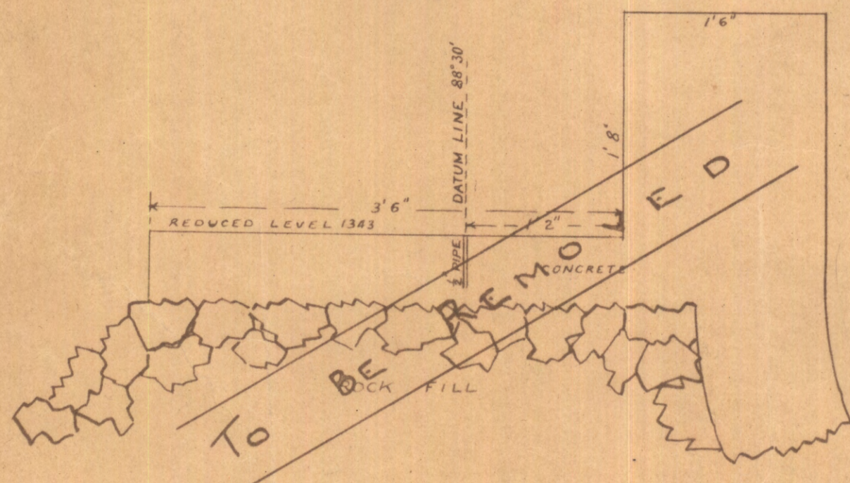
CROSS SECTION OF REMAINING PORTION OF ORIGINAL WALL.
