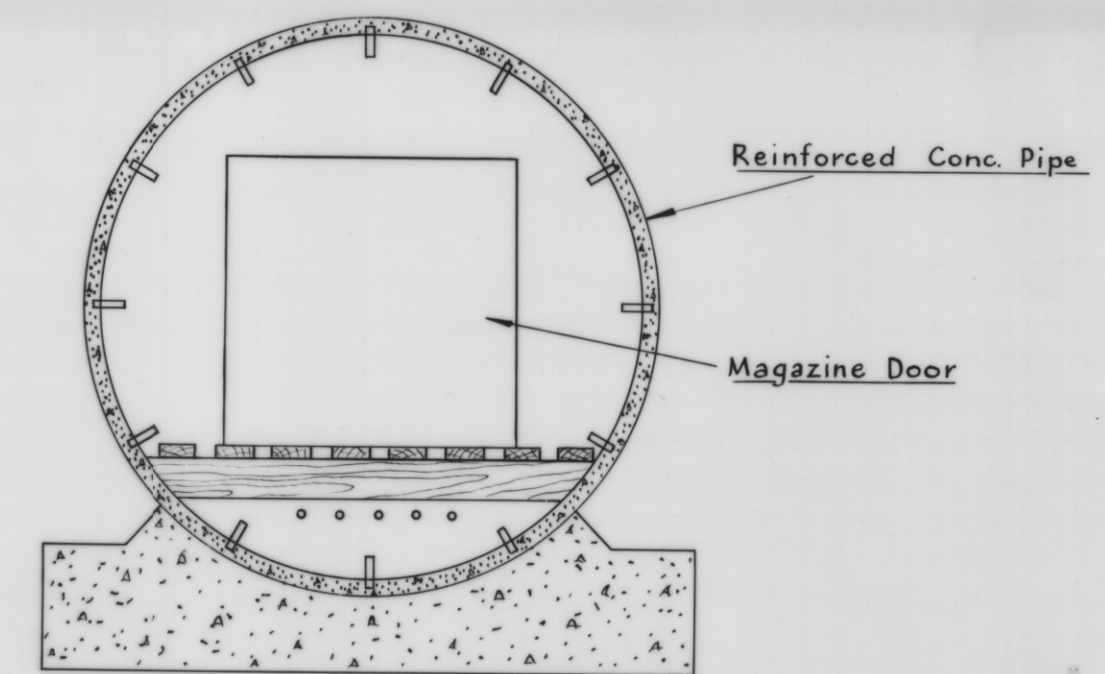
Section C-C
