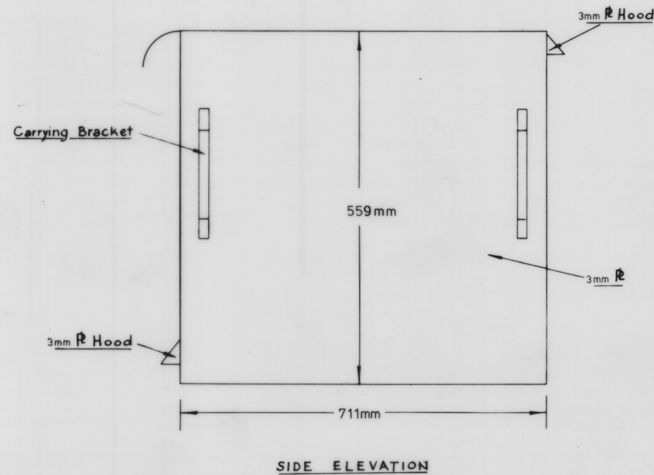
SIDE ELEVATION
