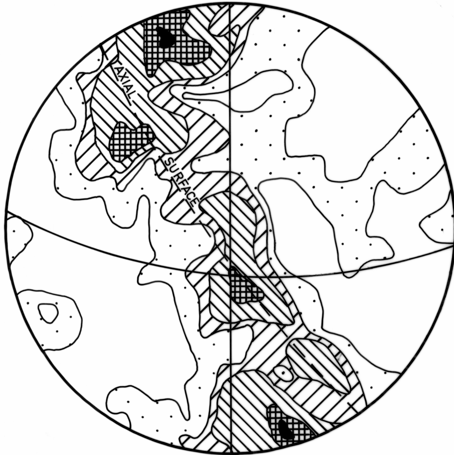
200 Quartz optic axes, section 39348 contours 0.25, 1.25, 2.25, 4.25, 5.75% per 1% area
