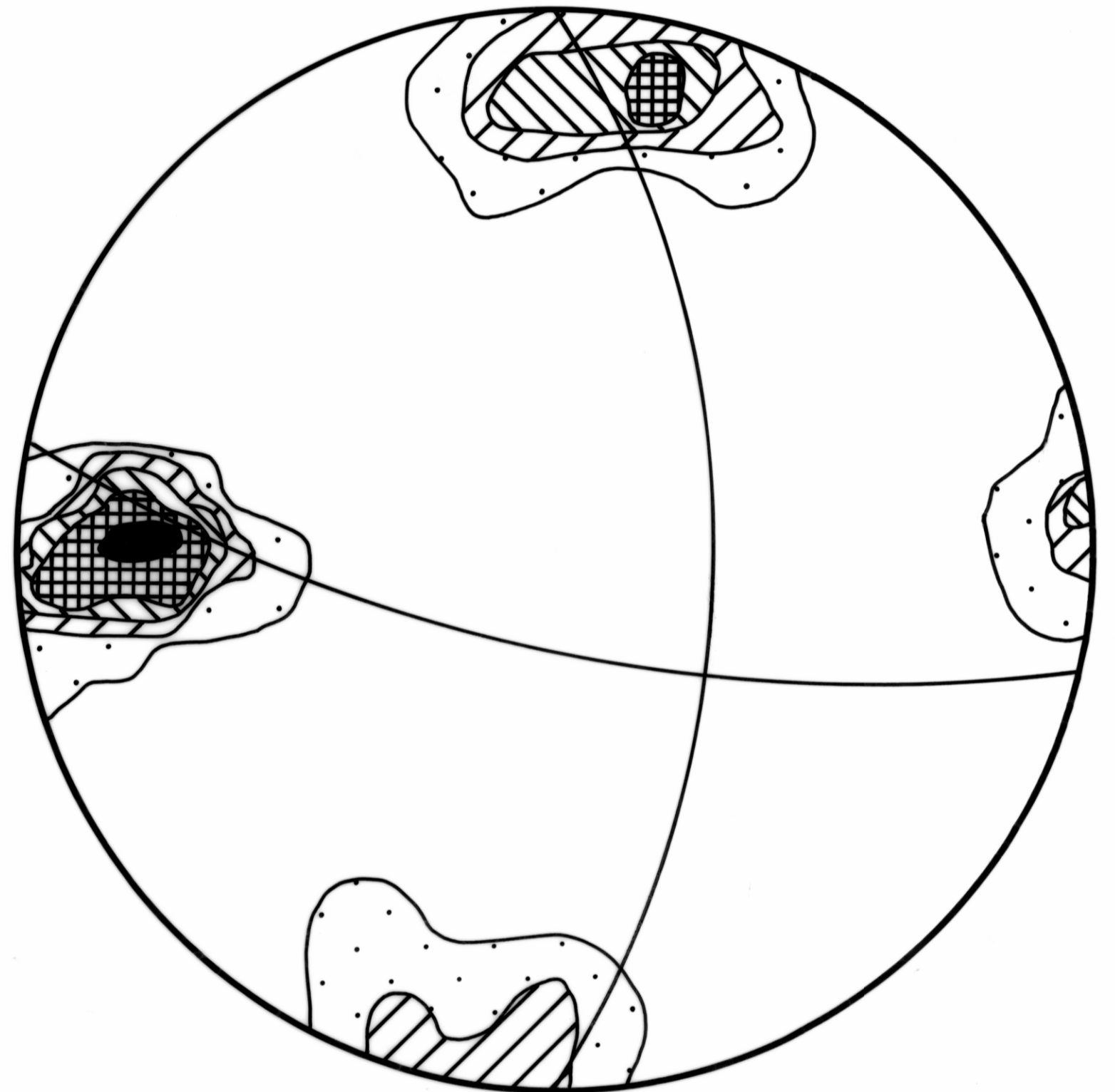
70 Foliation poles, section 39348 contours 0.7, 4, 8, 10, 20% per 1% area
