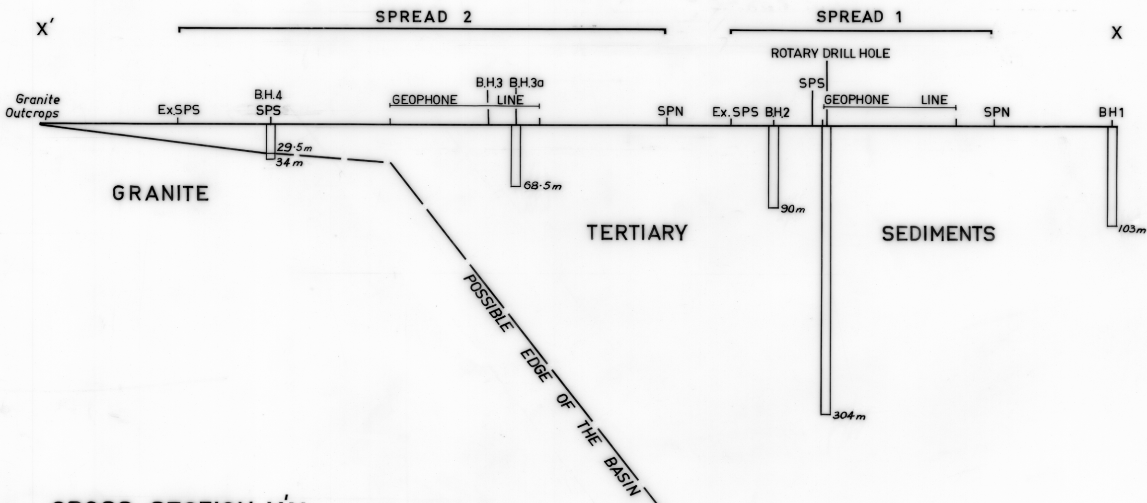
CROSS SECTION X'X
