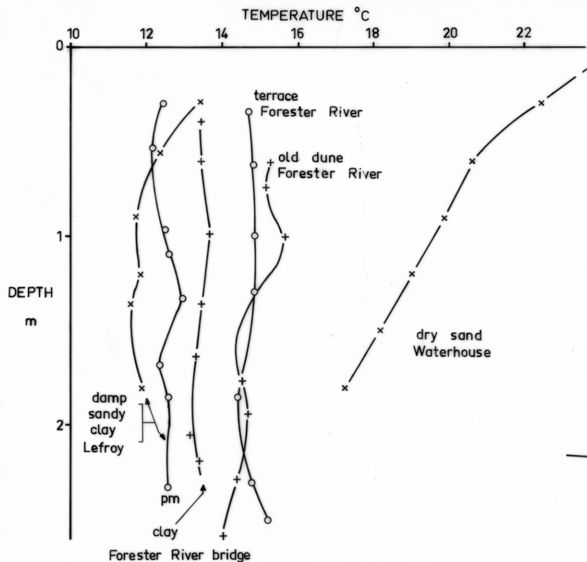
TYPICAL TEMPERATURE PROFILES
