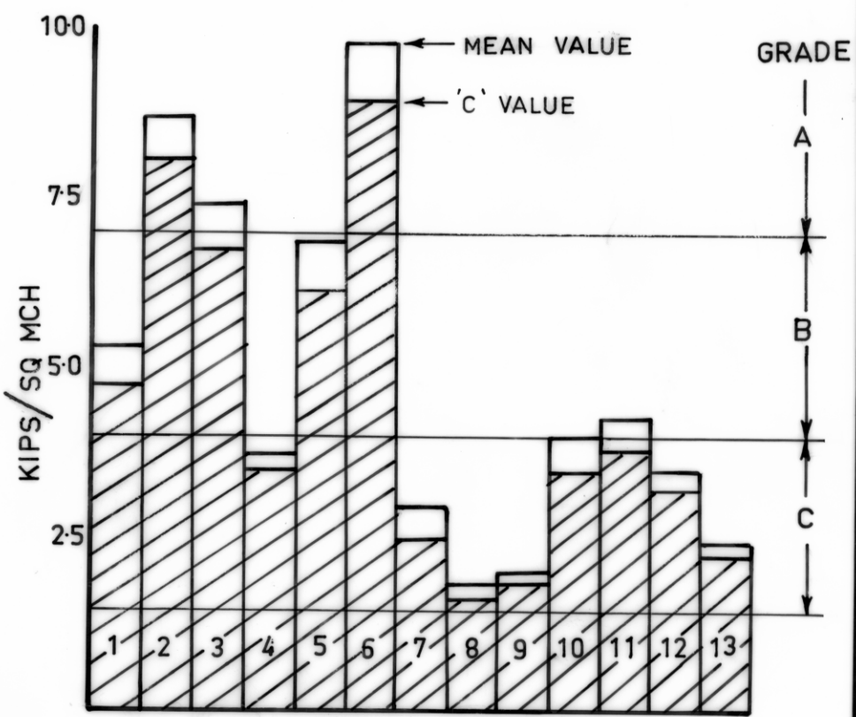
CRUSHING STRENGTH (1 KIP = 1000 LBS)
