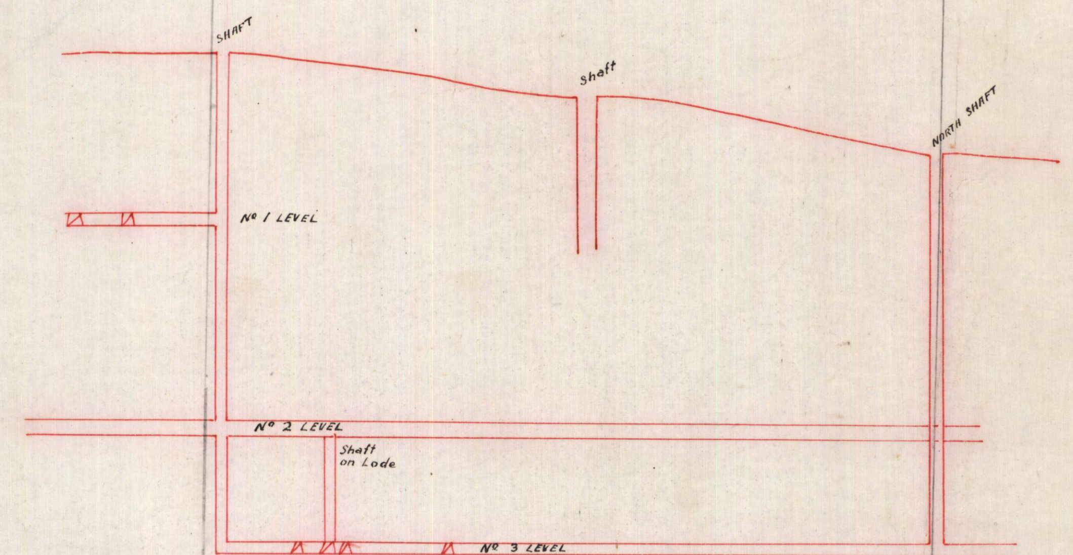
TRANSVERSE SECTION Projected on Plane bearing East-West
