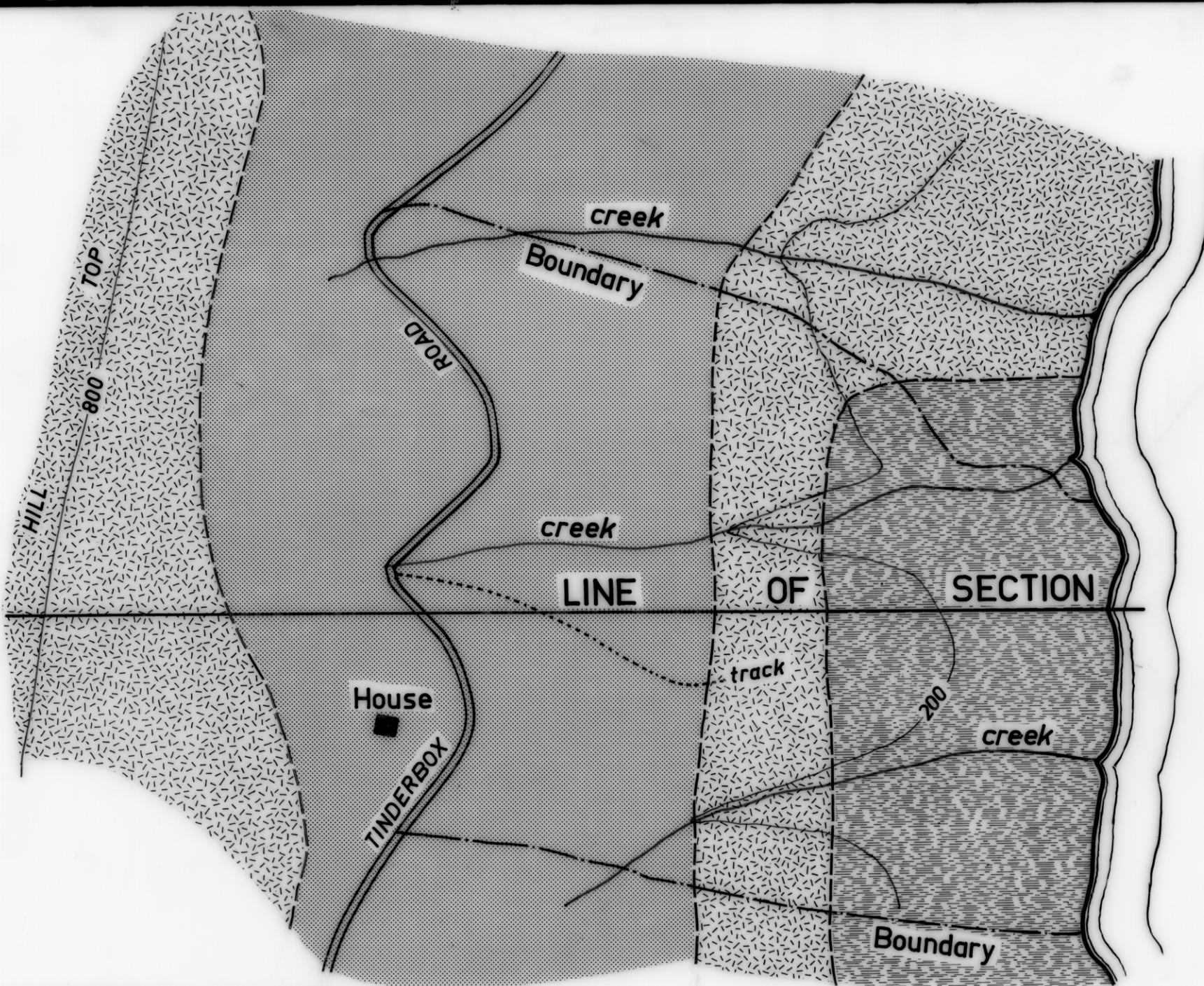
GEOLOGICAL SKETCH MAP Property owned by K.G. BROOKS
