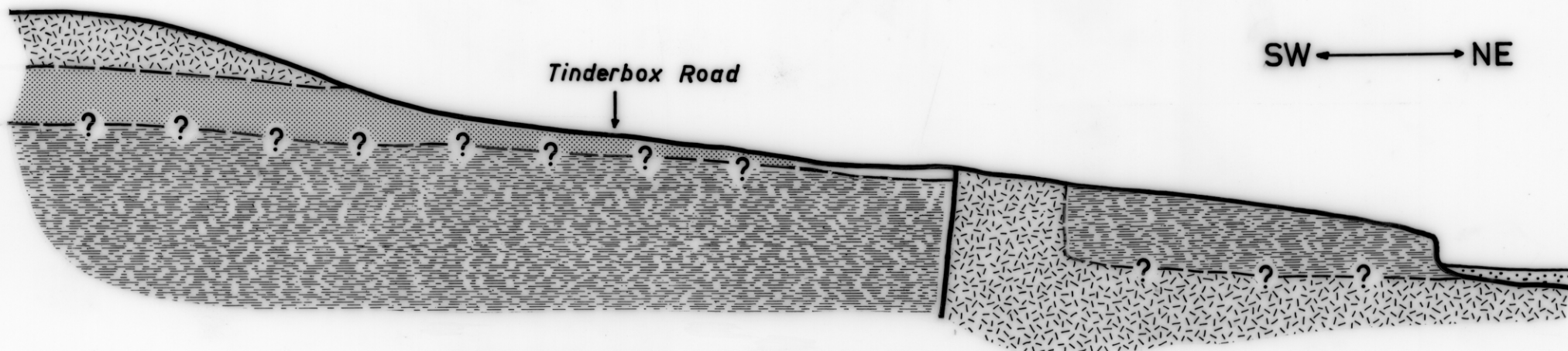
SECTION ACROSS BLOCK Natural scale
