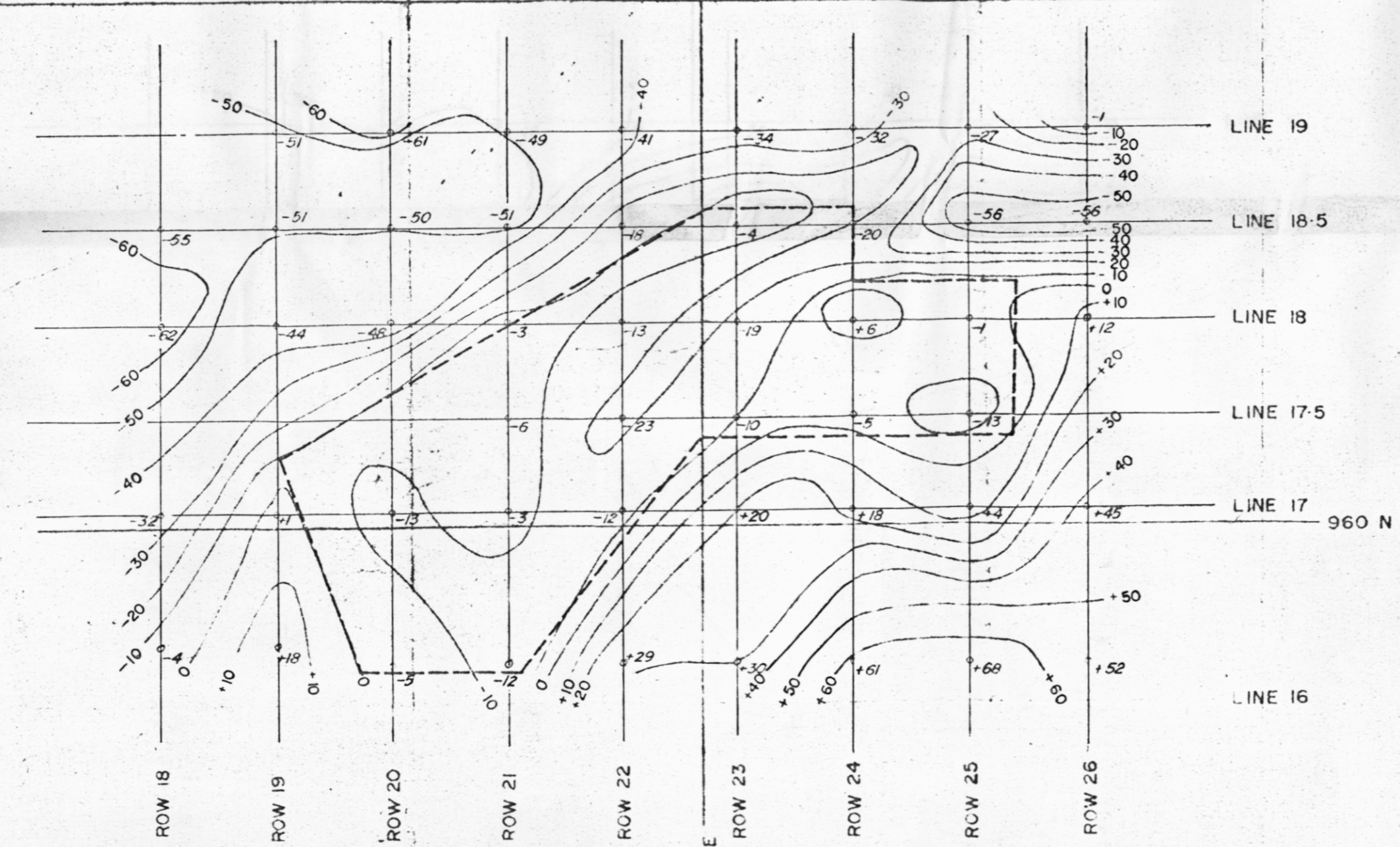
PLAN OF BOTTOM CONTOURS
