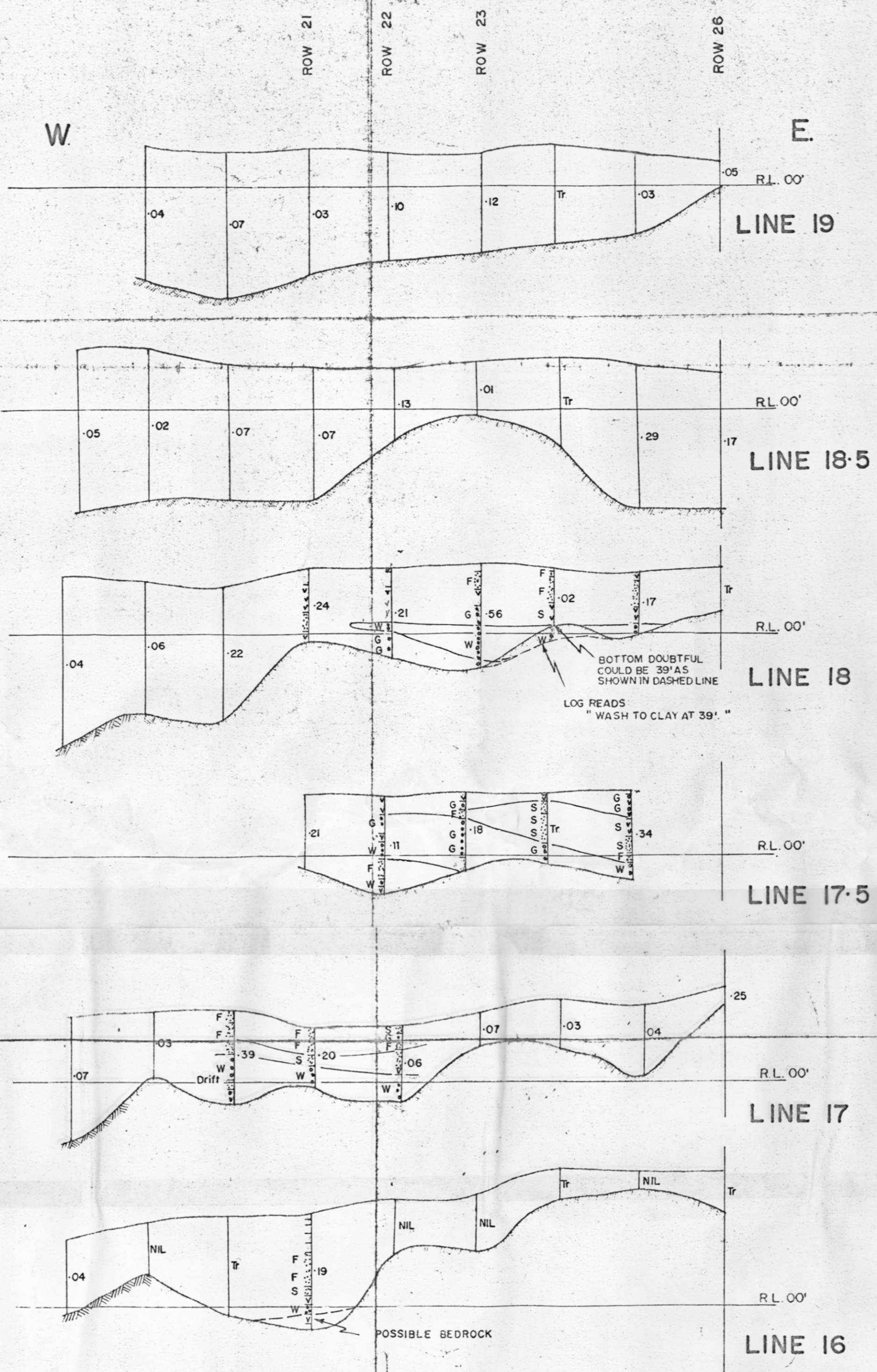
SECTIONS LOOKING NORTH THROUGH LINES 16, 17, 17.5, 18, 18.5 & 19.
