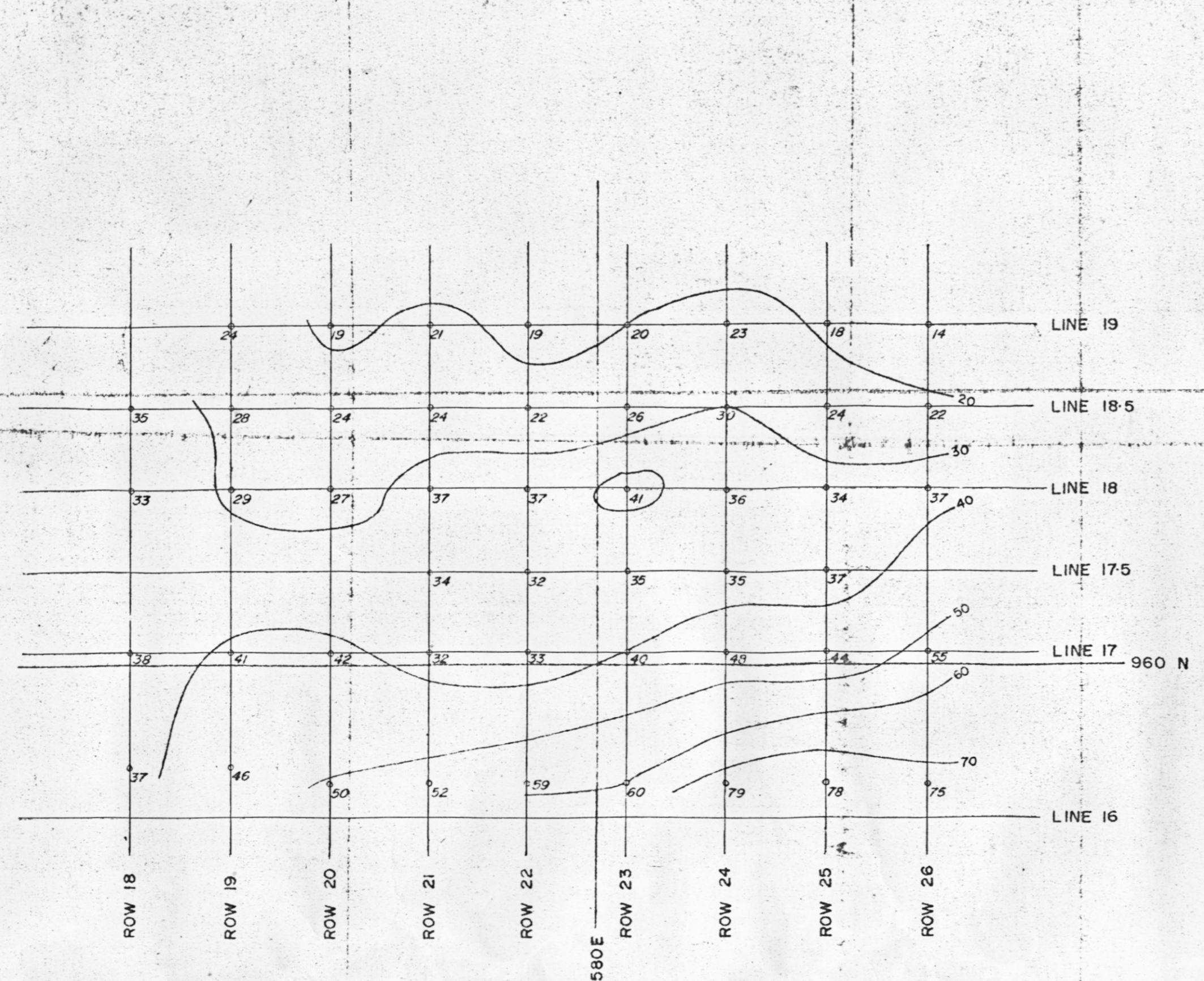
PLAN SURFACE CONTOURS (BASED ON REDUCED LEVELS OF DRILL HOLE COLLARS)
