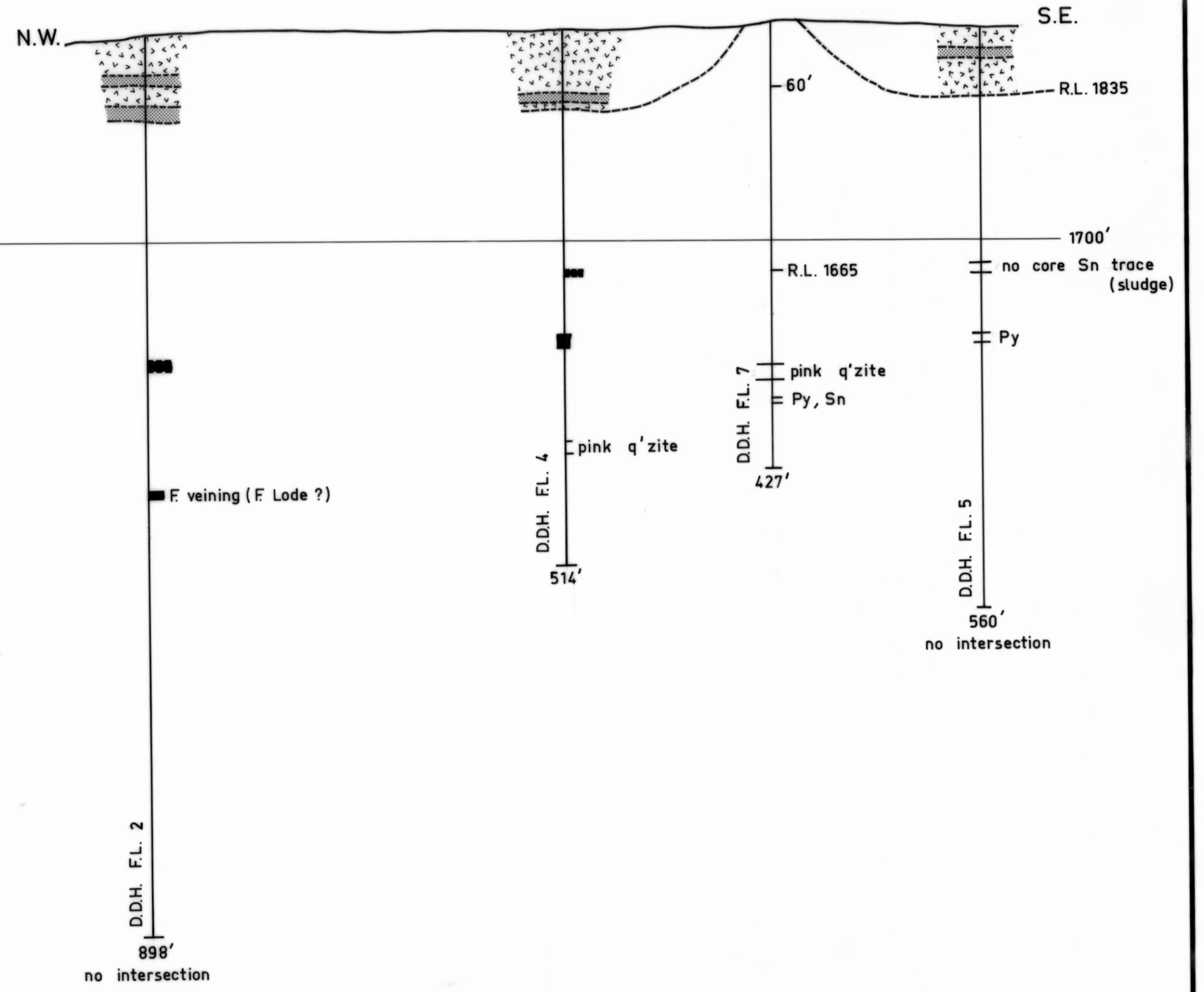
CROSS SECTION FL. 2 — FL. 5
