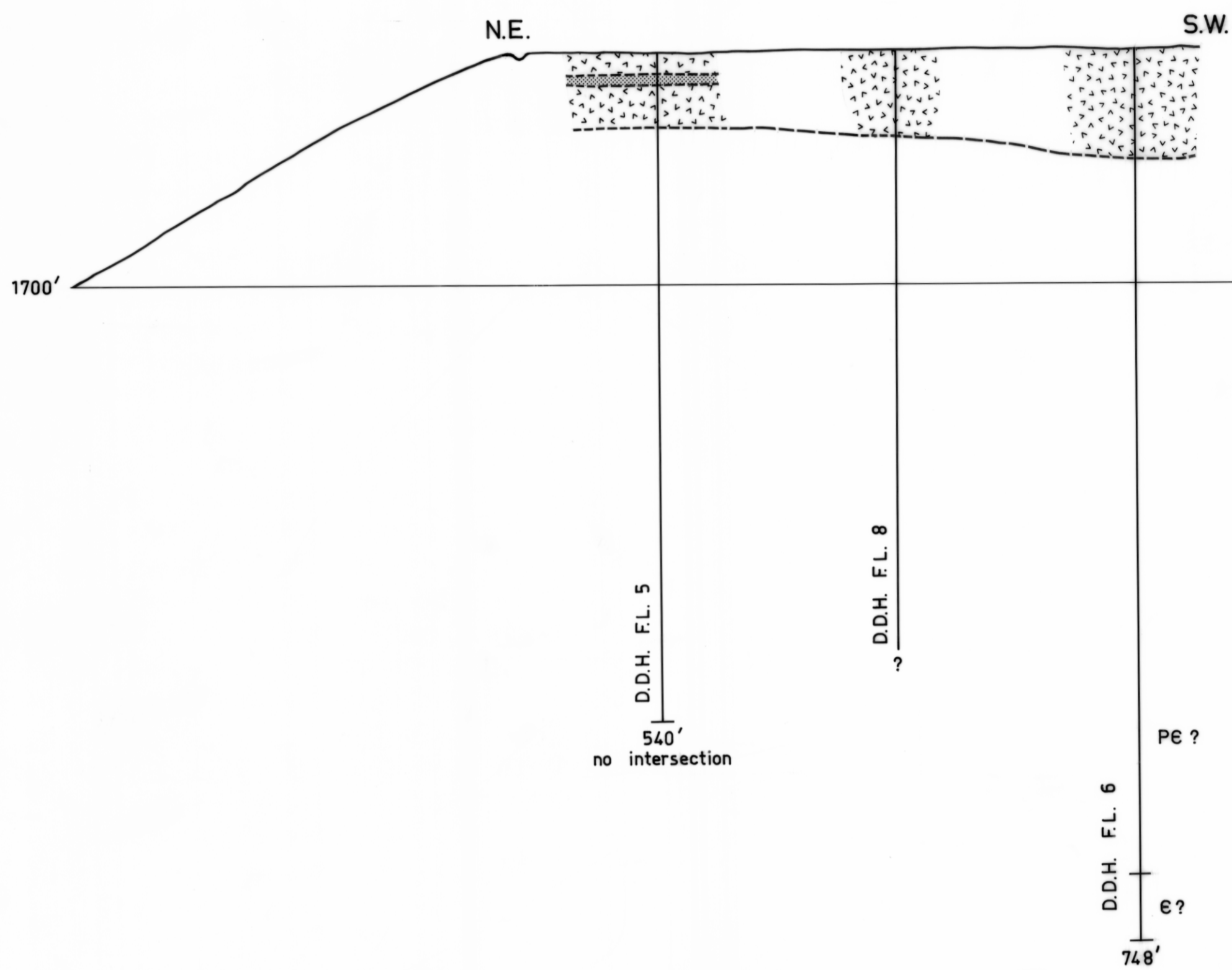
CROSS SECTION FL. 5 — FL. 6
