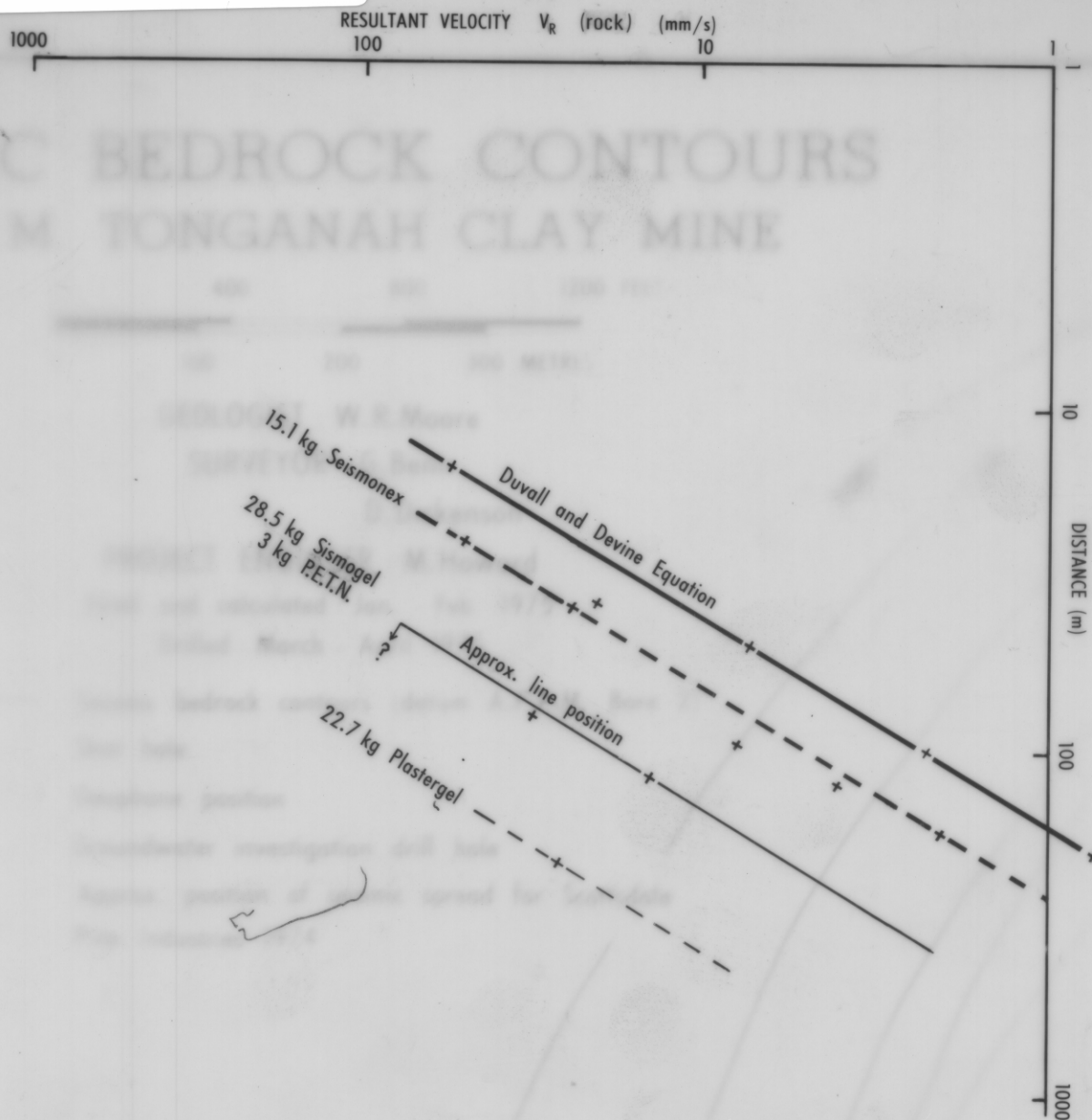
Figure 1 Rock Vibration Determinations
