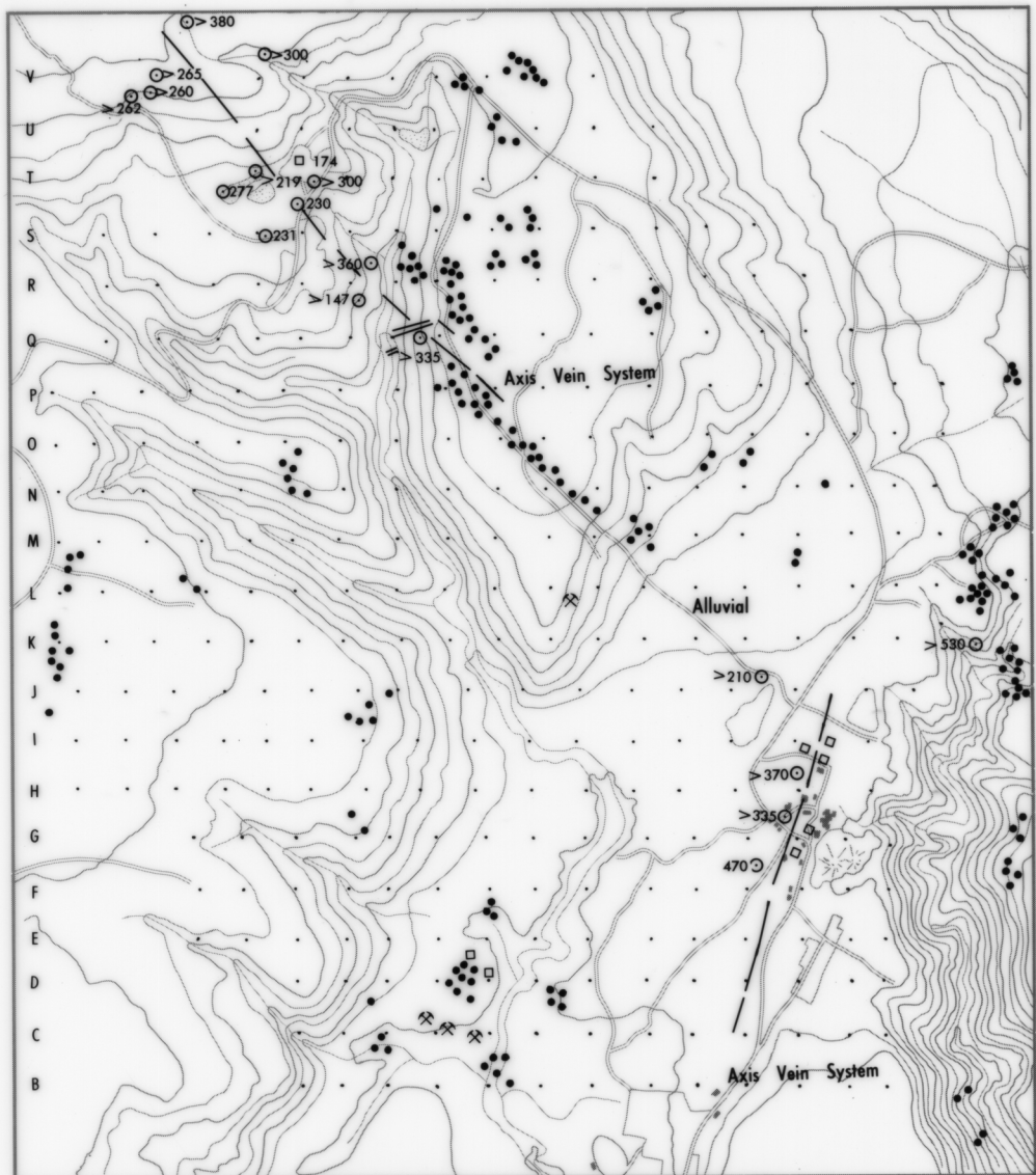
GRAVITY SURVEY ROSSARDEN - STOREYS CREEK AREA STRUCTURE AND MINE CONTROL INFORMATION □ Shaft ⊗ Workings • Vein outcrops (Quartz Rubble) ⊙ Depth to granite contact in metres (based on drilling or workings) Data supplied by Cominco Exploration Pty Ltd 0 150 300 m TASMANIA DEPARTMENT OF MINES
