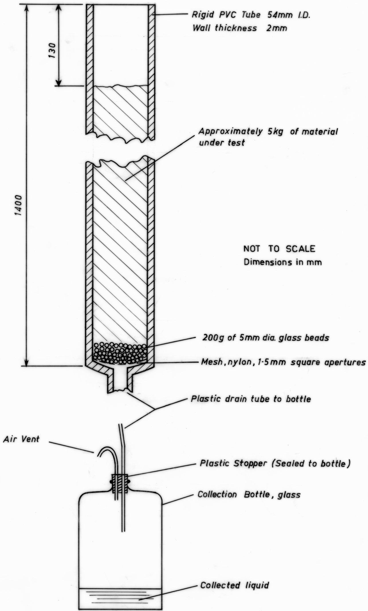
R680 SKETCH OF TEST APPARATUS
