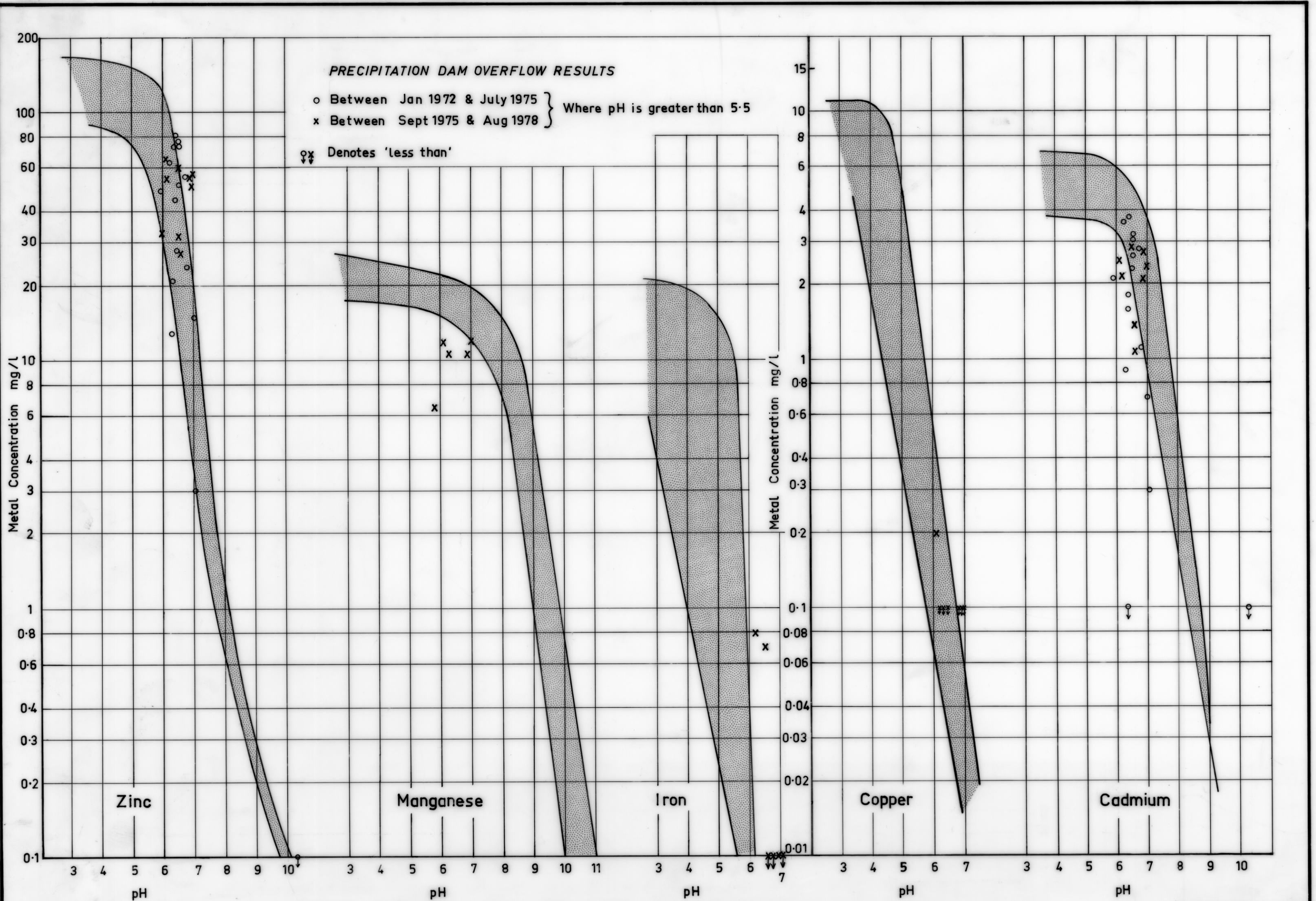
CURVES SHOWING CHANGES IN METAL CONCENTRATION WITH RISING pH ON STOREYS CREEK MINE WATER SAMPLES 737477, 740420, 741497 & 750887 SODA ASH USED TO RAISE pH.
