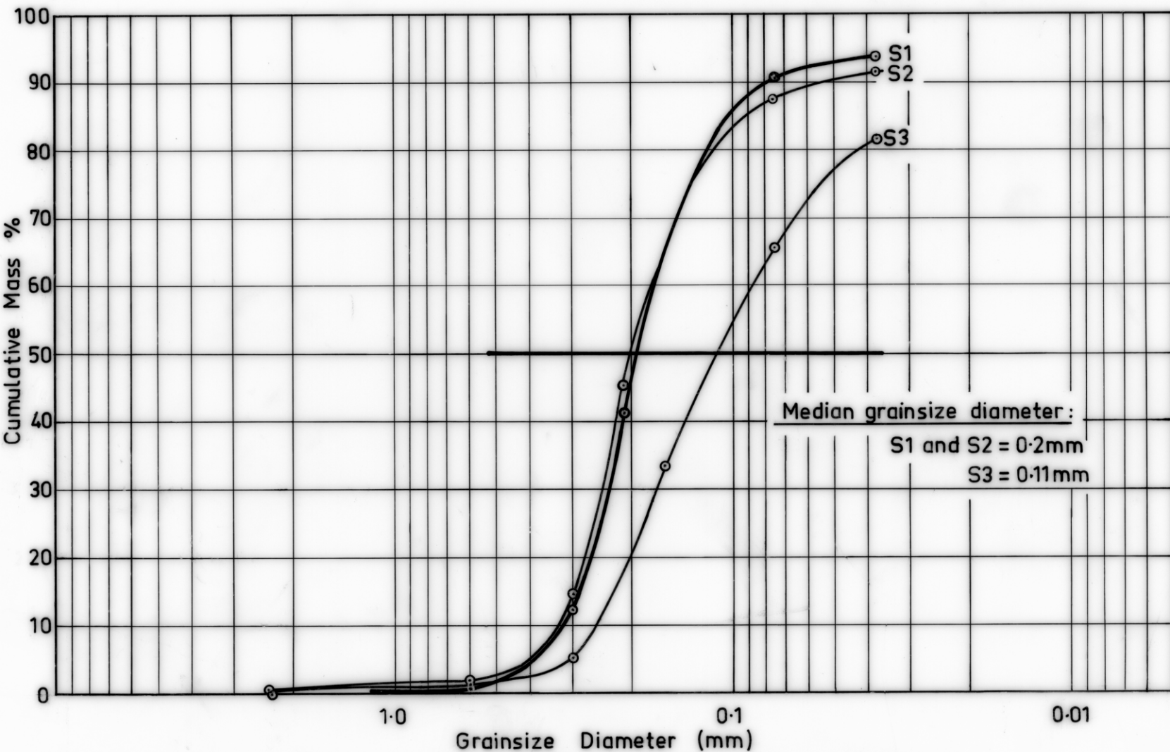
FIG. 4 GRAINSIZE ANALYSIS - PERTH NURSERY
