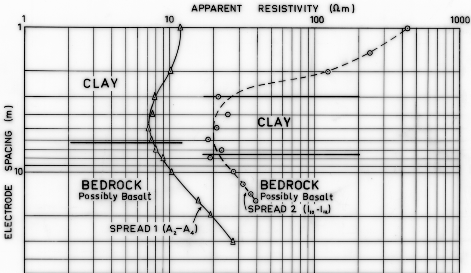
FIG. 2 RESISTIVITY SPREADS—PERTH NURSERY (WENNER CONFIGURATION)
