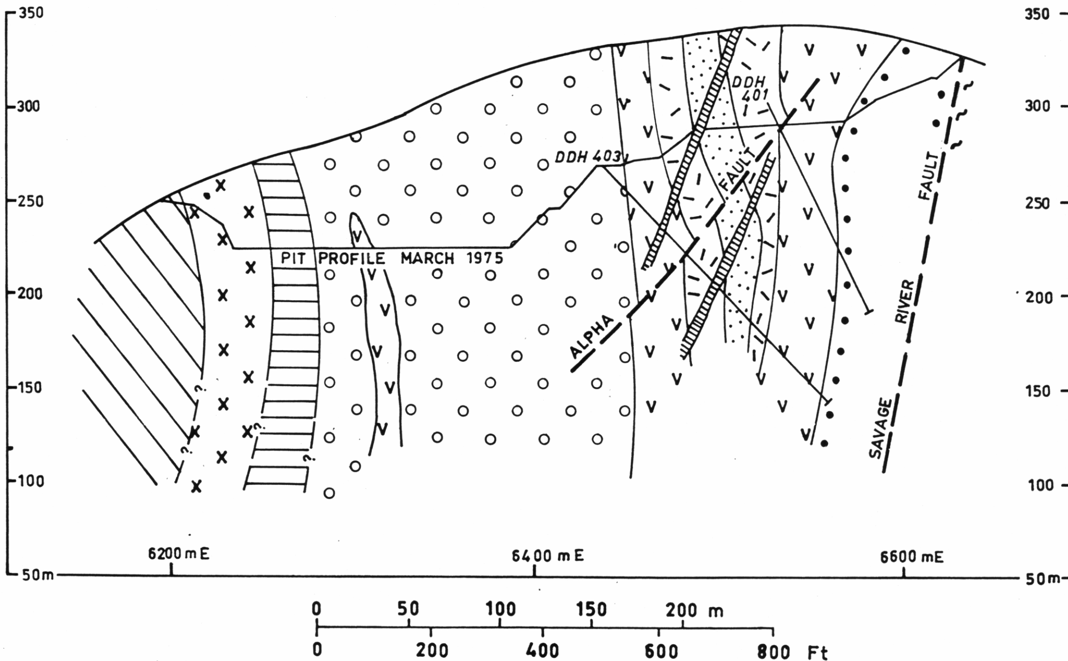
GEOLOGICAL CROSS SECTION AT 7000mN
