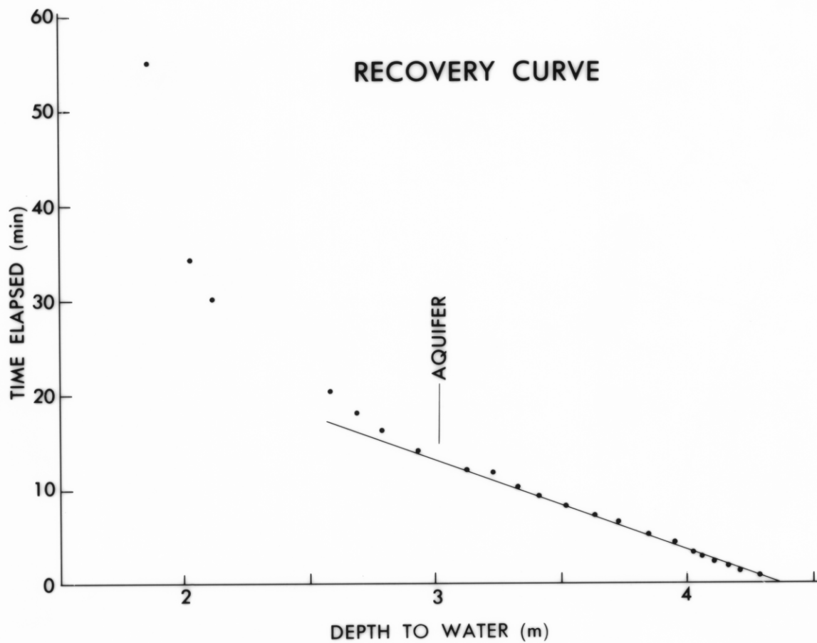
Figure 18 RECOVERY CURVES, BORE HOLE 13, ST LEONARDS
