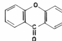
XANTHONE
