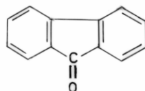
FLUORENE
