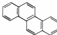
CHRYSENE
