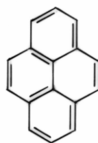
PYRENE
