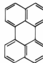
PARYLENE
