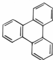
TRIPHENYLENE
