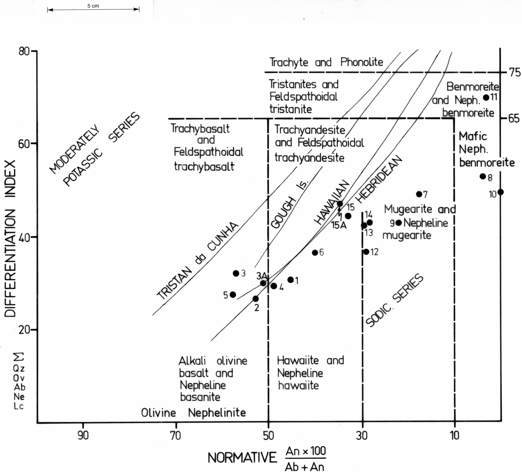
Figure 8. Chemical Variation Diagrams Hebridean Rocks
