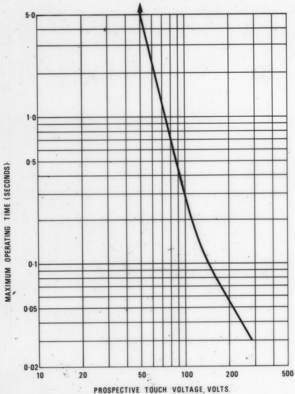
SYSTEMS UP TO 1000 VOLTS
