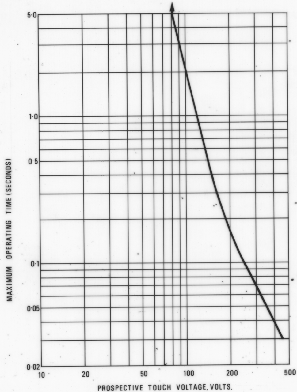
SYSTEMS ABOVE 1000 VOLTS
