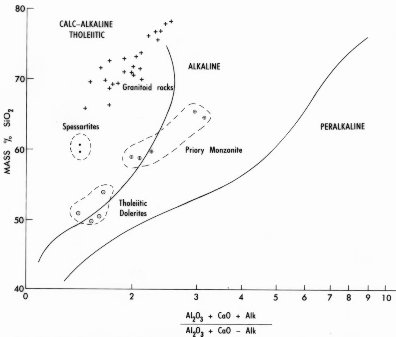
PLOT OF ALKALINITY RATIO AGAINST SiO 2 IN MASS PERCENT (WRIGHT 1969) SHOWING ANOMALOUS DISTRIBUTION OF THE PRIORY MONZONITE
