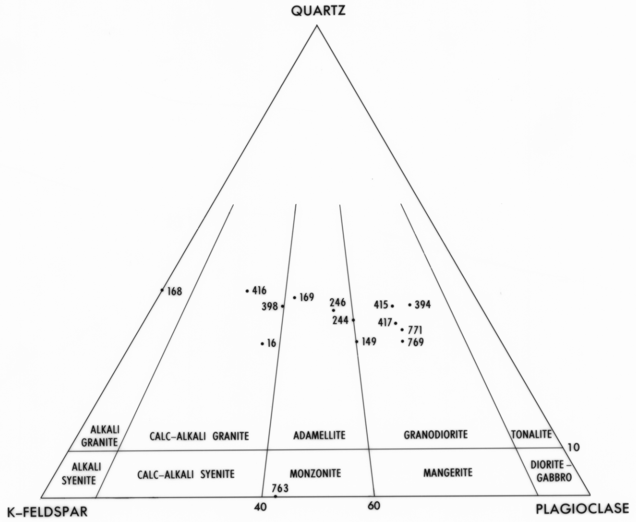
ROCK CLASSIFICATION FROM MODAL ANALYSIS A TRIANGULAR DIAGRAM IN TERMS OF QUARTZ, K-FELDSPAR AND PLAGIOCLASE TASMANIA DEPARTMENT OF MINES, JULY 1976 GEOLOGIST: J.D. COCKER DRAWN: J.S. LADANIWSKYJ 4161
