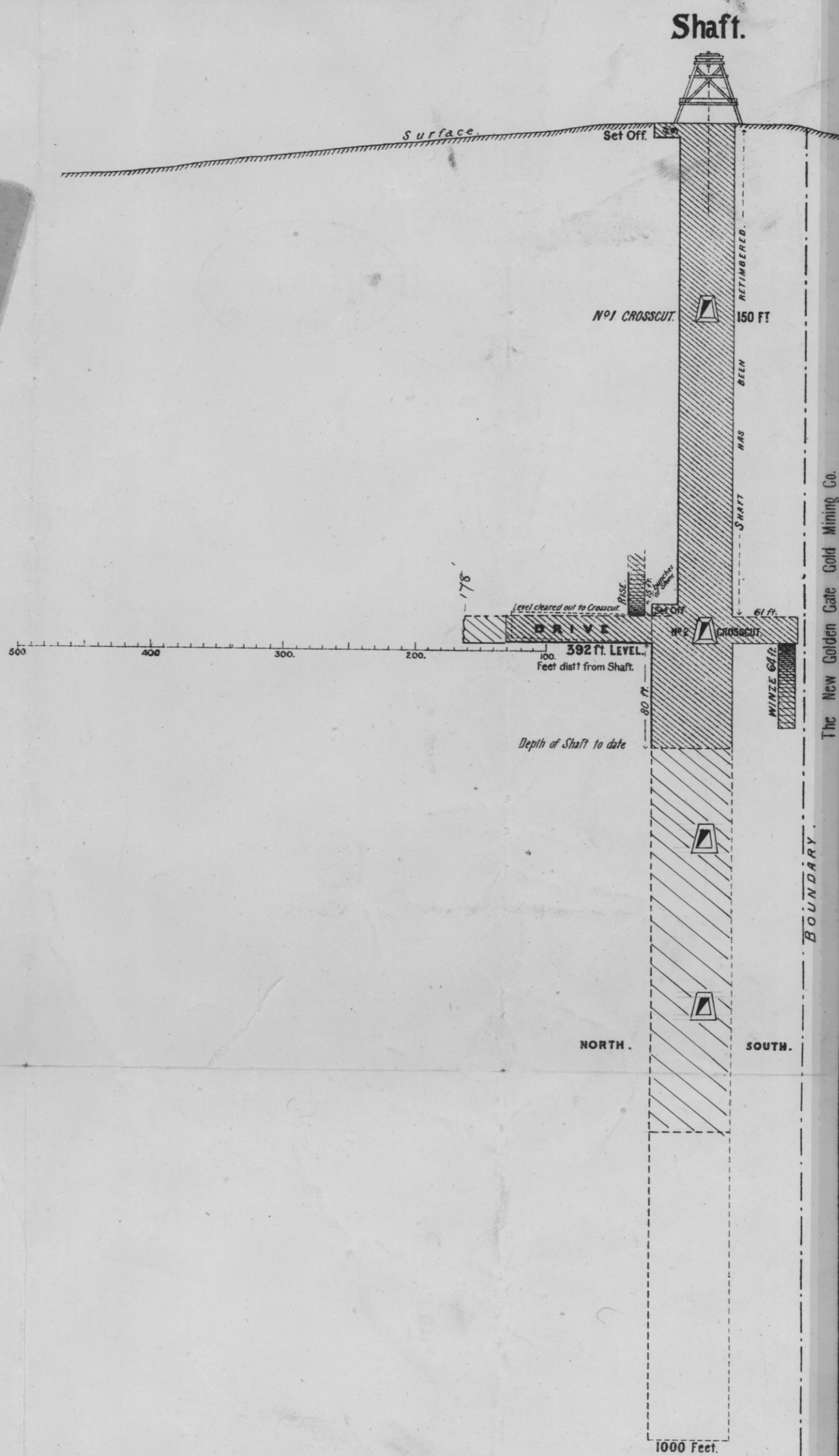
— LONGITUDINAL SECTION — — Looking East —
