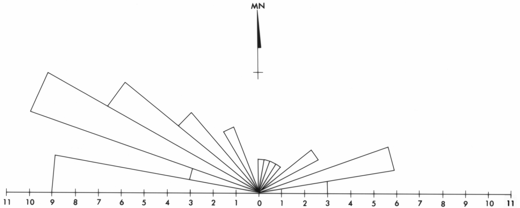
ROSE DIAGRAM OF STRIKE DIRECTIONS OF MUSCOVITE -ANDALUSITE DYKES ST HELENS ISLAND - ST HELENS POINT AREA
