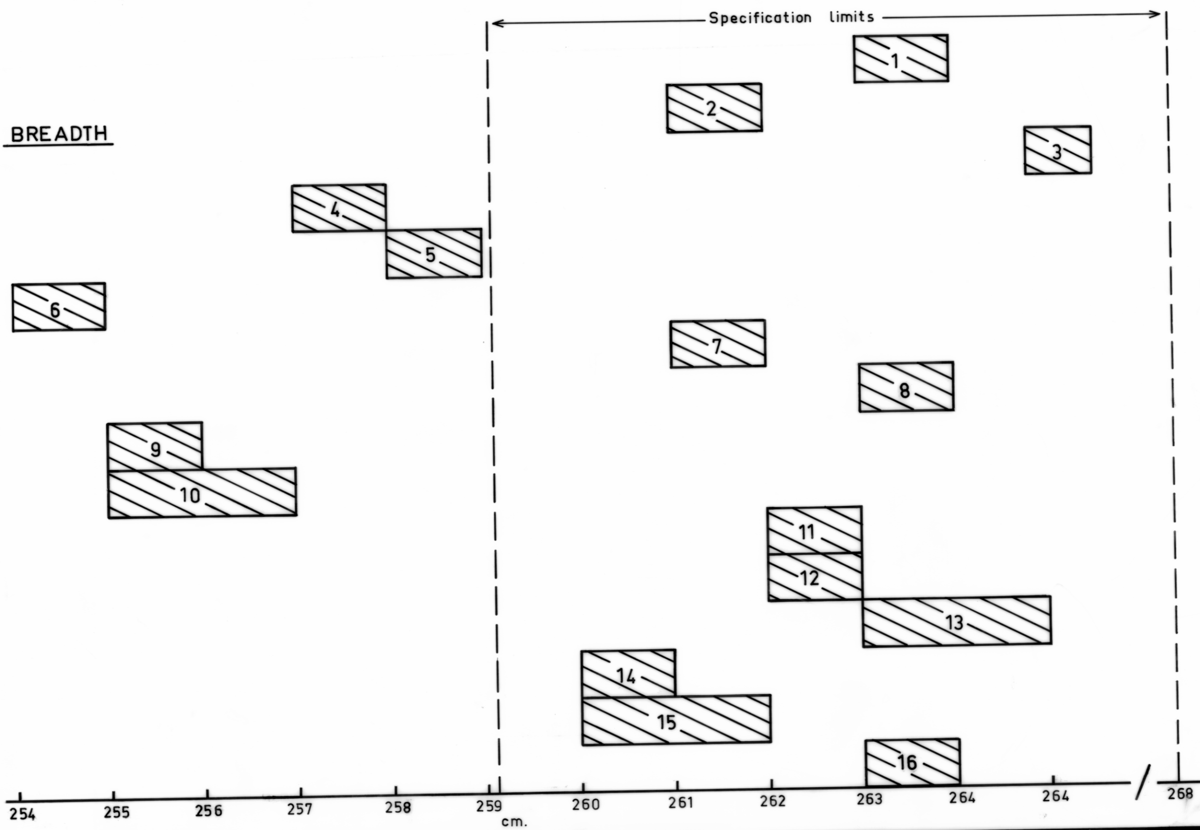
COMPARISON OF BRICK DIMENSIONS WITH SPECIFICATION REQUIREMENTS R743 (DEC 1976)
