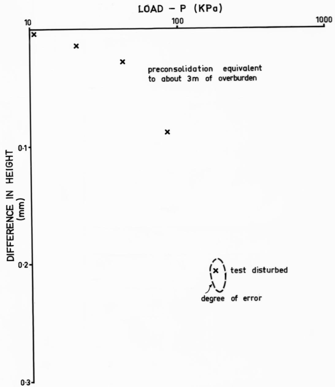
Consolidation test on a sample of brown clay from 14 Norwood Avenue, Tarooma. Sample from hole P8, depth 0.85m.
